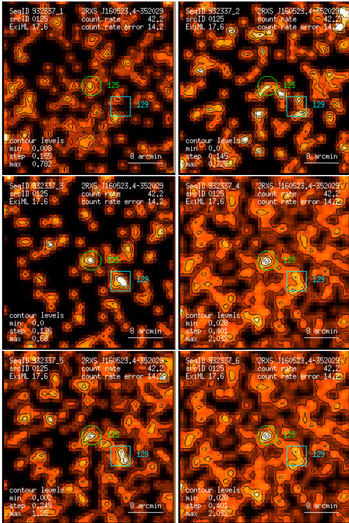
Figure 125: RASS 932337: detection 0125: band rate images, Gaussian filter: (1) PSPC channels 11 – 41, (2) 52 – 90, (3) 91 – 201, (4) 11 – 235, (5) 52 – 201, (6) 11 – 201. Broad band rates in counts/ks. Band rate contour levels in counts/ks/arcmin 2 .
