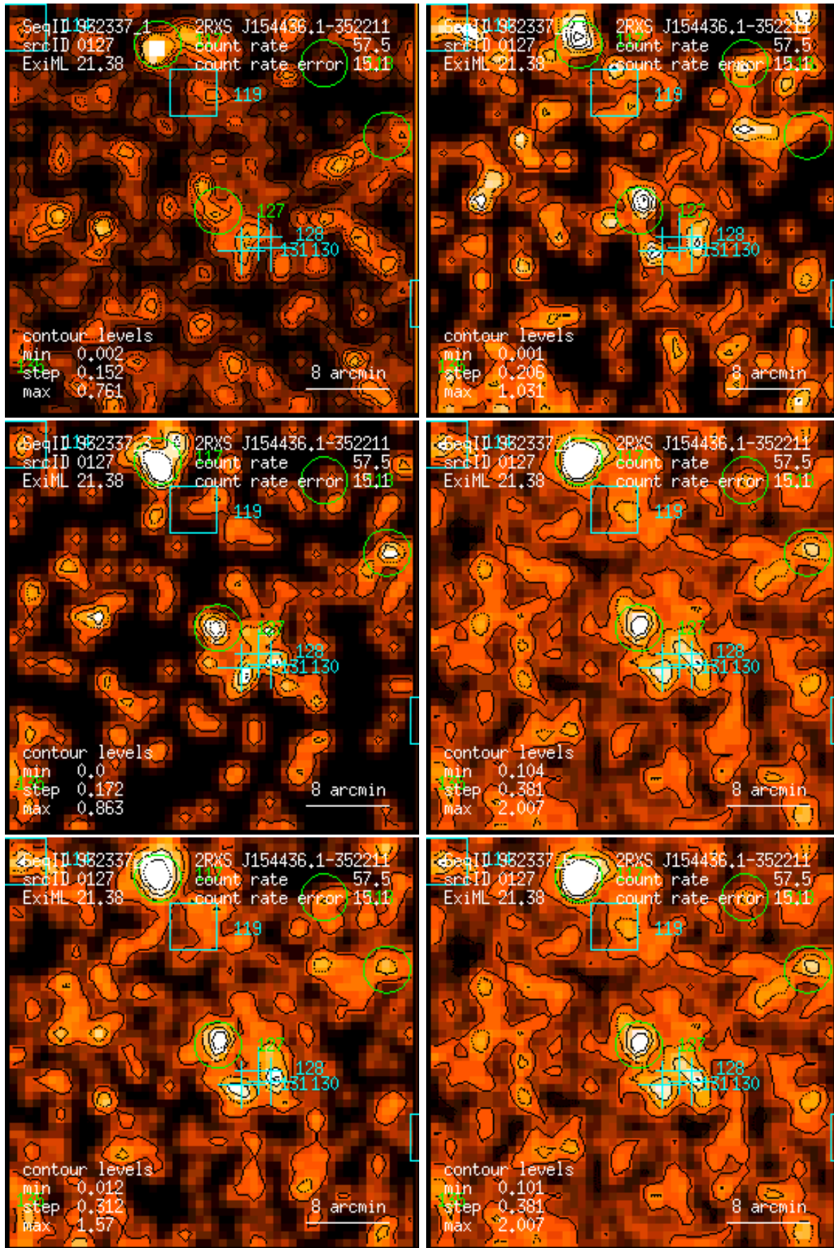
Figure 127: RASS 932337: detection 0127: band rate images, Gaussian filter: (1) PSPC channels 11 – 41, (2) 52 – 90, (3) 91 – 201, (4) 11 – 235, (5) 52 – 201, (6) 11 – 201. Broad band rates in counts/ks. Band rate contour levels in counts/ks/arcmin 2 .
