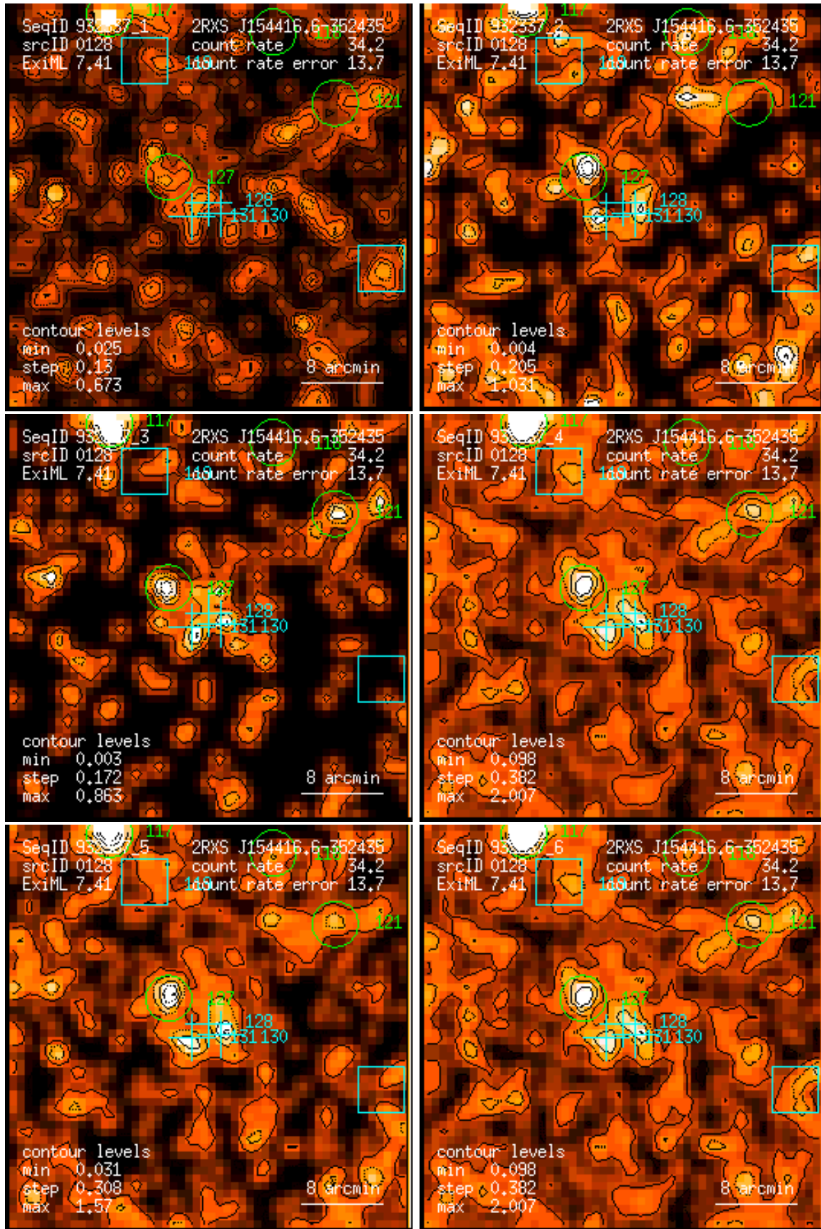
Figure 128: RASS 932337: detection 0128: band rate images, Gaussian filter: (1) PSPC channels 11 – 41, (2) 52 – 90, (3) 91 – 201, (4) 11 – 235, (5) 52 – 201, (6) 11 – 201. Broad band rates in counts/ks. Band rate contour levels in counts/ks/arcmin 2 .
