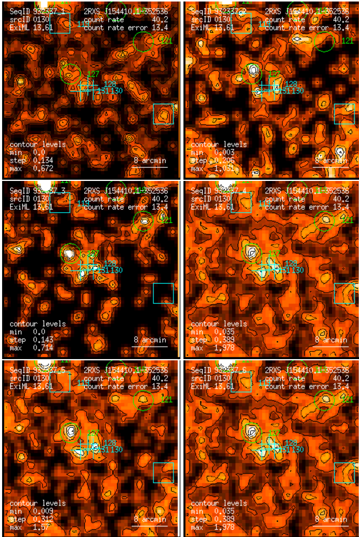
Figure 130: RASS 932337: detection 0130: band rate images, Gaussian filter: (1) PSPC channels 11 – 41, (2) 52 – 90, (3) 91 – 201, (4) 11 – 235, (5) 52 – 201, (6) 11 – 201. Broad band rates in counts/ks. Band rate contour levels in counts/ks/arcmin 2 .
