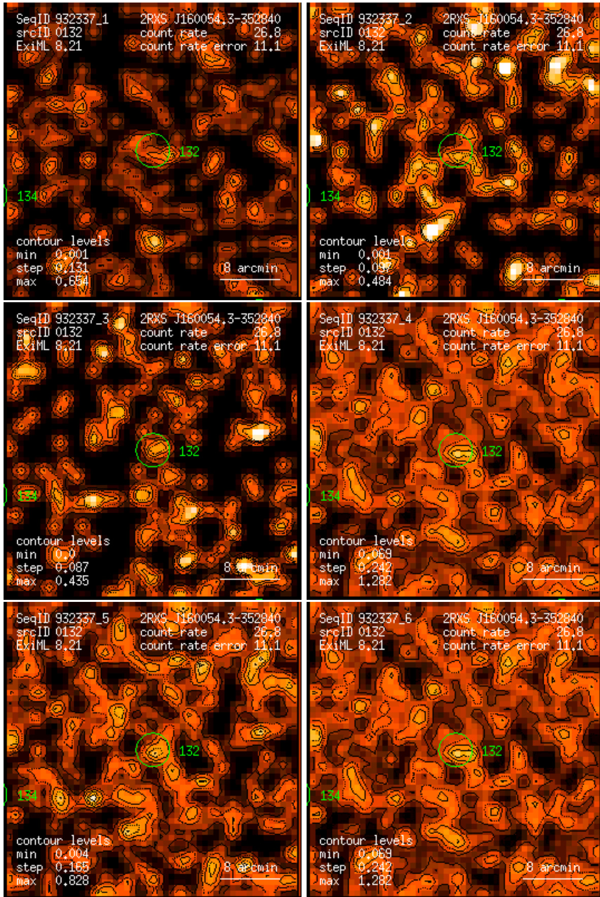
Figure 132: RASS 932337: detection 0132: band rate images, Gaussian filter: (1) PSPC channels 11 – 41, (2) 52 – 90, (3) 91 – 201, (4) 11 – 235, (5) 52 – 201, (6) 11 – 201. Broad band rates in counts/ks. Band rate contour levels in counts/ks/arcmin 2 .
