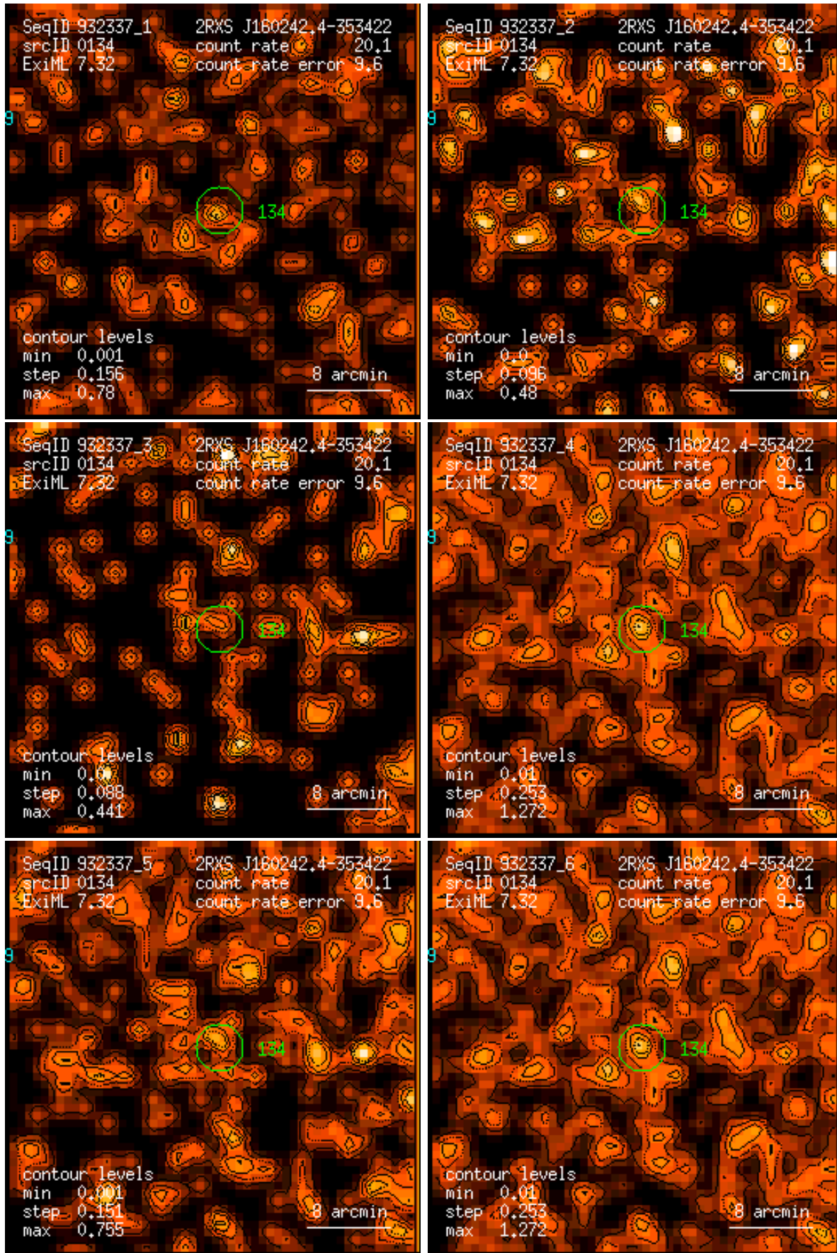
Figure 134: RASS 932337: detection 0134: band rate images, Gaussian filter: (1) PSPC channels 11 – 41, (2) 52 – 90, (3) 91 – 201, (4) 11 – 235, (5) 52 – 201, (6) 11 – 201. Broad band rates in counts/ks. Band rate contour levels in counts/ks/arcmin 2 .
