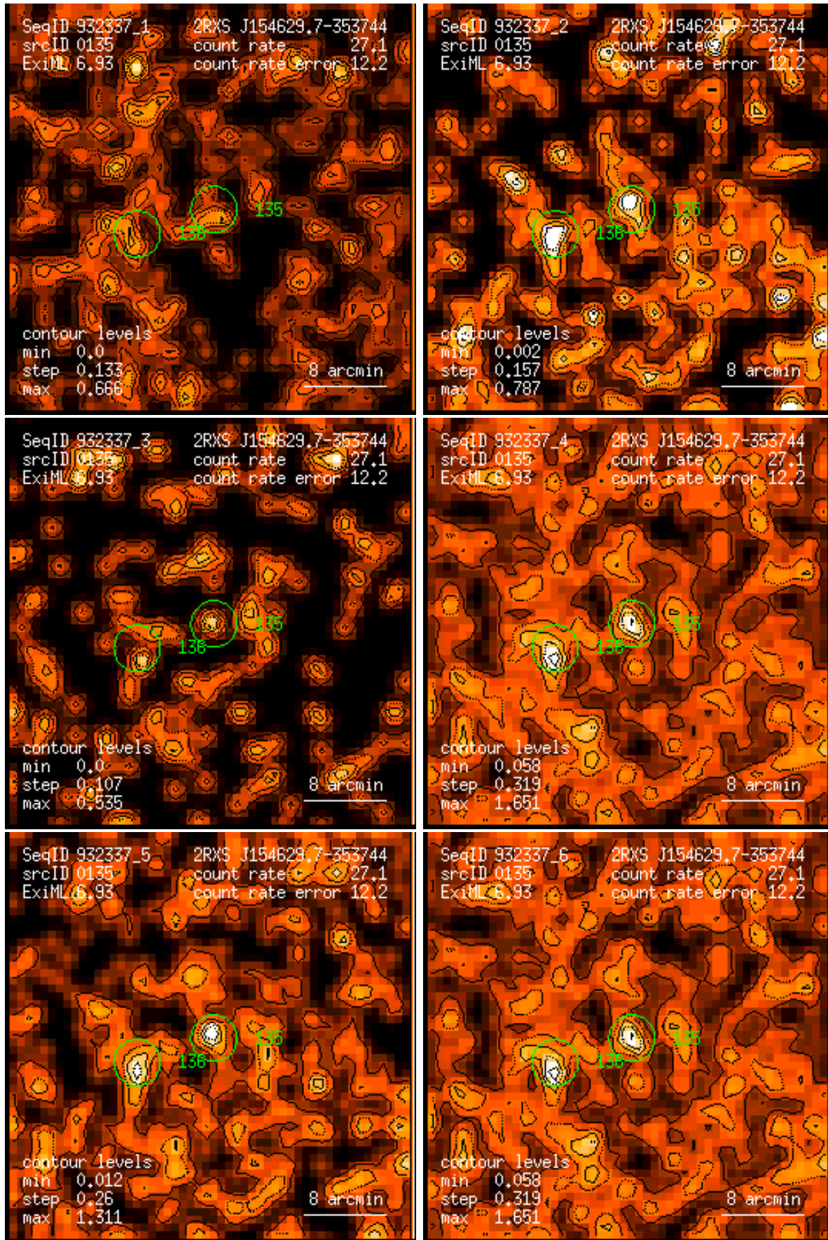
Figure 135: RASS 932337: detection 0135: band rate images, Gaussian filter: (1) PSPC channels 11 – 41, (2) 52 – 90, (3) 91 – 201, (4) 11 – 235, (5) 52 – 201, (6) 11 – 201. Broad band rates in counts/ks. Band rate contour levels in counts/ks/arcmin 2 .
