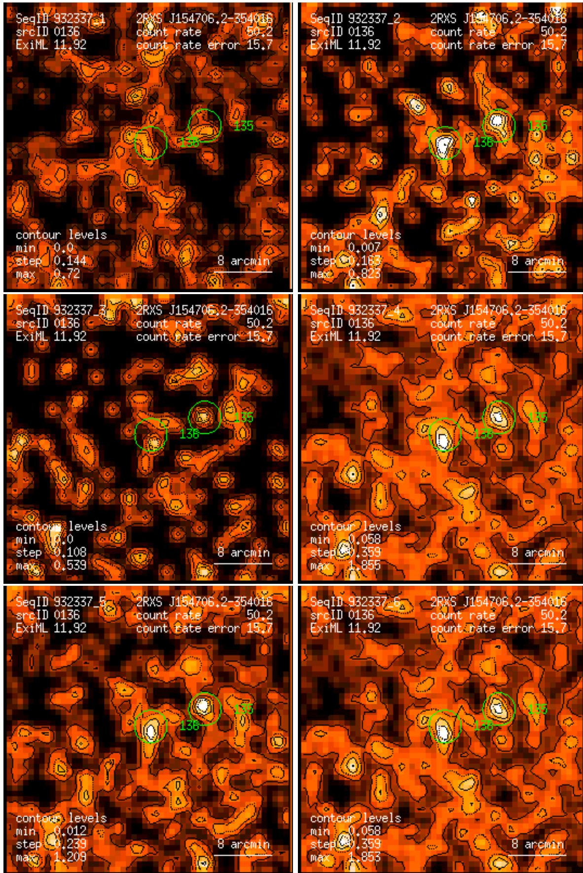
Figure 136: RASS 932337: detection 0136: band rate images, Gaussian filter: (1) PSPC channels 11 – 41, (2) 52 – 90, (3) 91 – 201, (4) 11 – 235, (5) 52 – 201, (6) 11 – 201. Broad band rates in counts/ks. Band rate contour levels in counts/ks/arcmin 2 .
