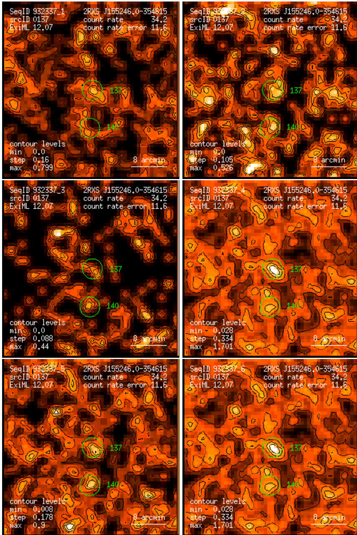
Figure 137: RASS 932337: detection 0137: band rate images, Gaussian filter: (1) PSPC channels 11 – 41, (2) 52 – 90, (3) 91 – 201, (4) 11 – 235, (5) 52 – 201, (6) 11 – 201. Broad band rates in counts/ks. Band rate contour levels in counts/ks/arcmin 2 .
