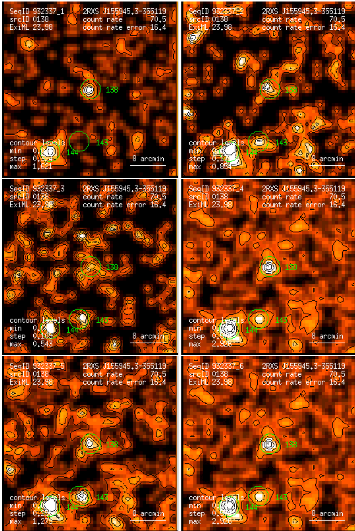
Figure 138: RASS 932337: detection 0138: band rate images, Gaussian filter: (1) PSPC channels 11 – 41, (2) 52 – 90, (3) 91 – 201, (4) 11 – 235, (5) 52 – 201, (6) 11 – 201. Broad band rates in counts/ks. Band rate contour levels in counts/ks/arcmin 2 .
