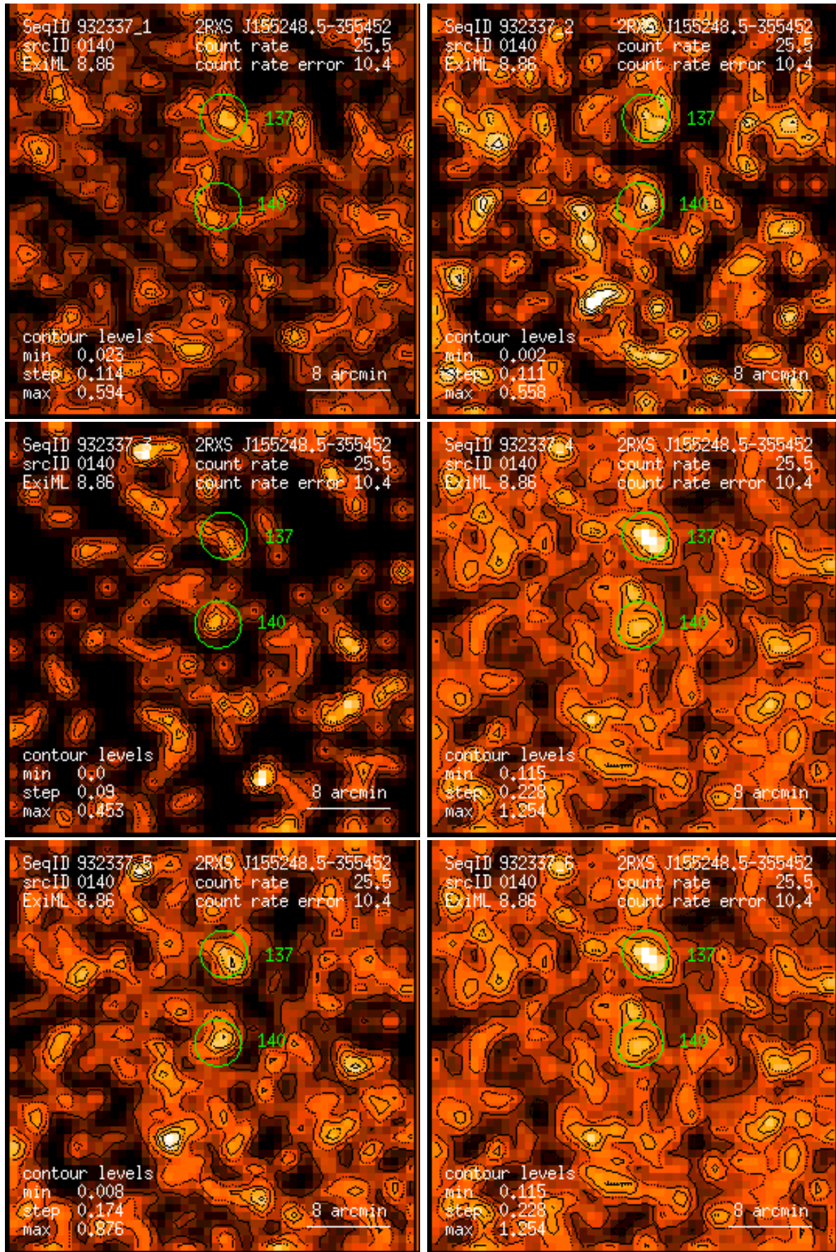
Figure 140: RASS 932337: detection 0140: band rate images, Gaussian filter: (1) PSPC channels 11 – 41, (2) 52 – 90, (3) 91 – 201, (4) 11 – 235, (5) 52 – 201, (6) 11 – 201. Broad band rates in counts/ks. Band rate contour levels in counts/ks/arcmin 2 .
