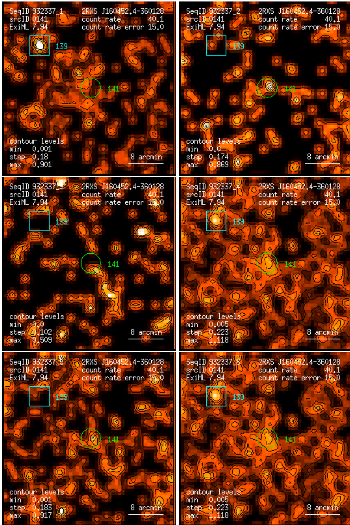
Figure 141: RASS 932337: detection 0141: band rate images, Gaussian filter: (1) PSPC channels 11 – 41, (2) 52 – 90, (3) 91 – 201, (4) 11 – 235, (5) 52 – 201, (6) 11 – 201. Broad band rates in counts/ks. Band rate contour levels in counts/ks/arcmin 2 .
