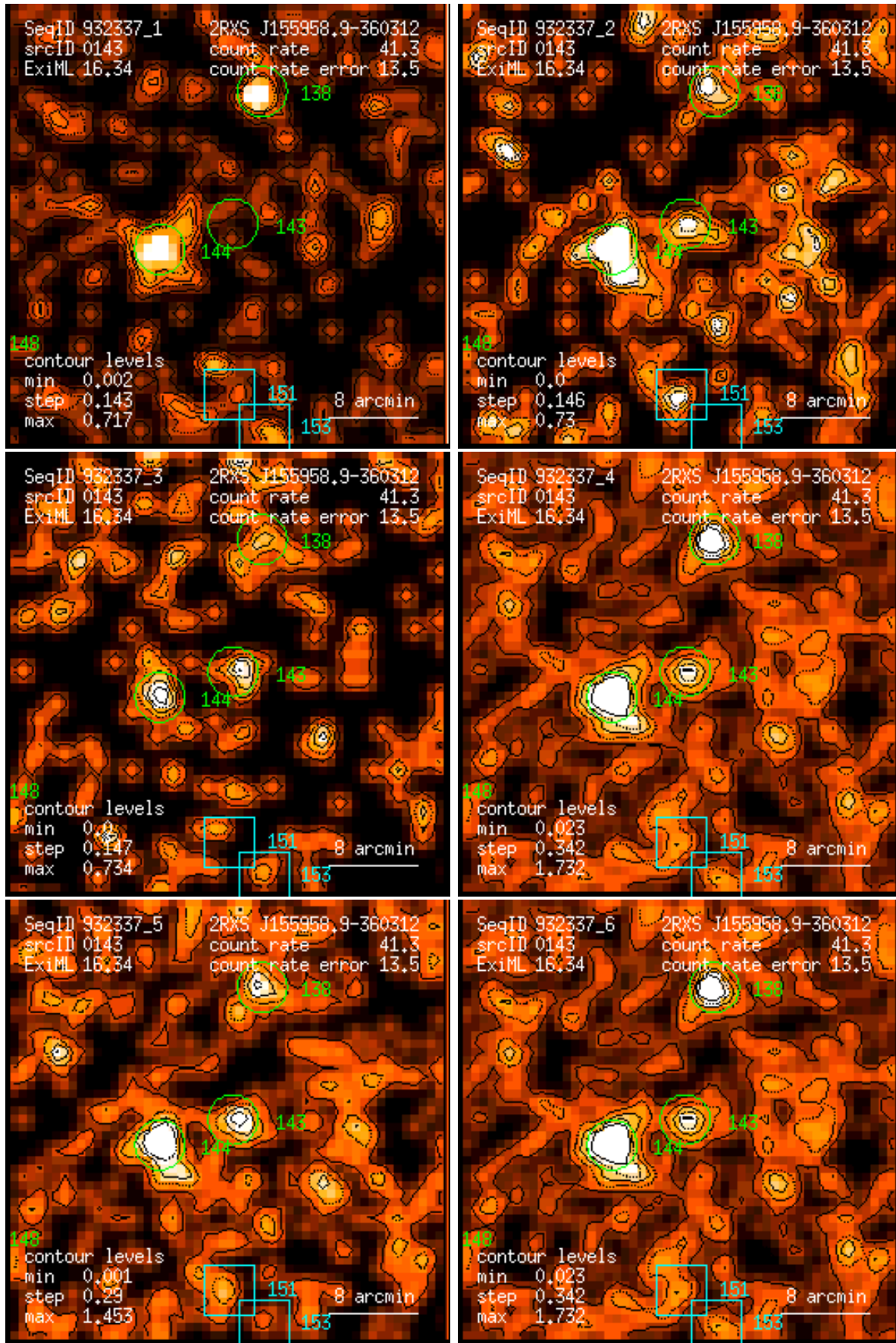
Figure 143: RASS 932337: detection 0143: band rate images, Gaussian filter: (1) PSPC channels 11 – 41, (2) 52 – 90, (3) 91 – 201, (4) 11 – 235, (5) 52 – 201, (6) 11 – 201. Broad band rates in counts/ks. Band rate contour levels in counts/ks/arcmin 2 .
