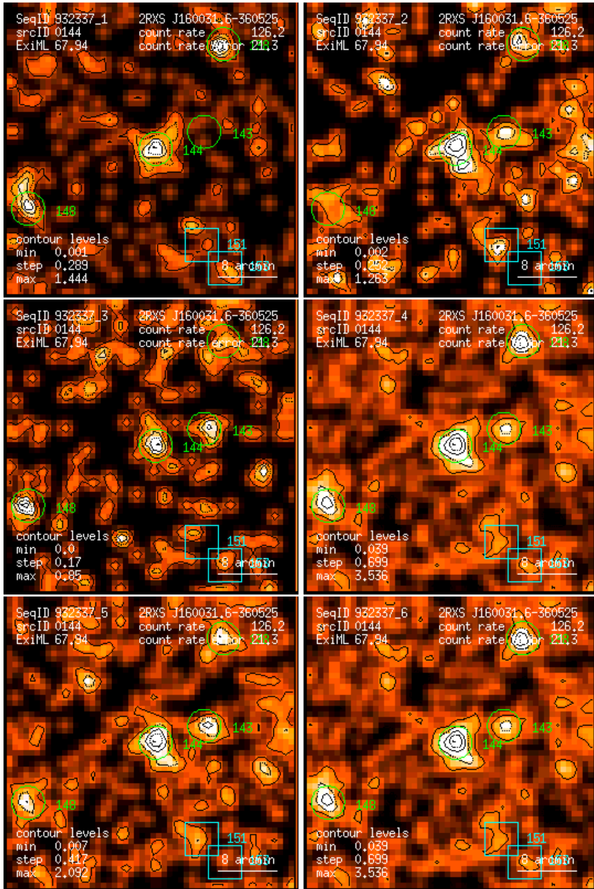
Figure 144: RASS 932337: detection 0144: band rate images, Gaussian filter: (1) PSPC channels 11 – 41, (2) 52 – 90, (3) 91 – 201, (4) 11 – 235, (5) 52 – 201, (6) 11 – 201. Broad band rates in counts/ks. Band rate contour levels in counts/ks/arcmin 2 .
