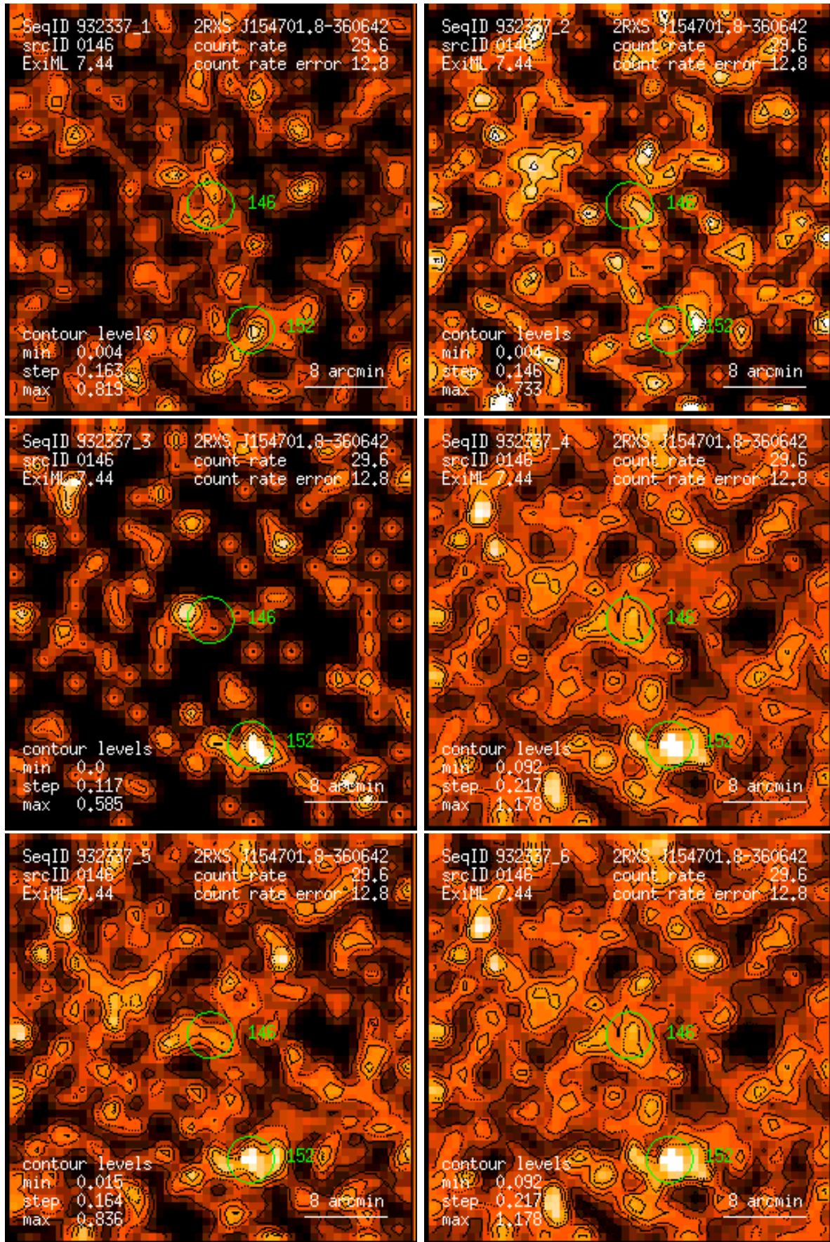
Figure 146: RASS 932337: detection 0146: band rate images, Gaussian filter: (1) PSPC channels 11 – 41, (2) 52 – 90, (3) 91 – 201, (4) 11 – 235, (5) 52 – 201, (6) 11 – 201. Broad band rates in counts/ks. Band rate contour levels in counts/ks/arcmin 2 .
