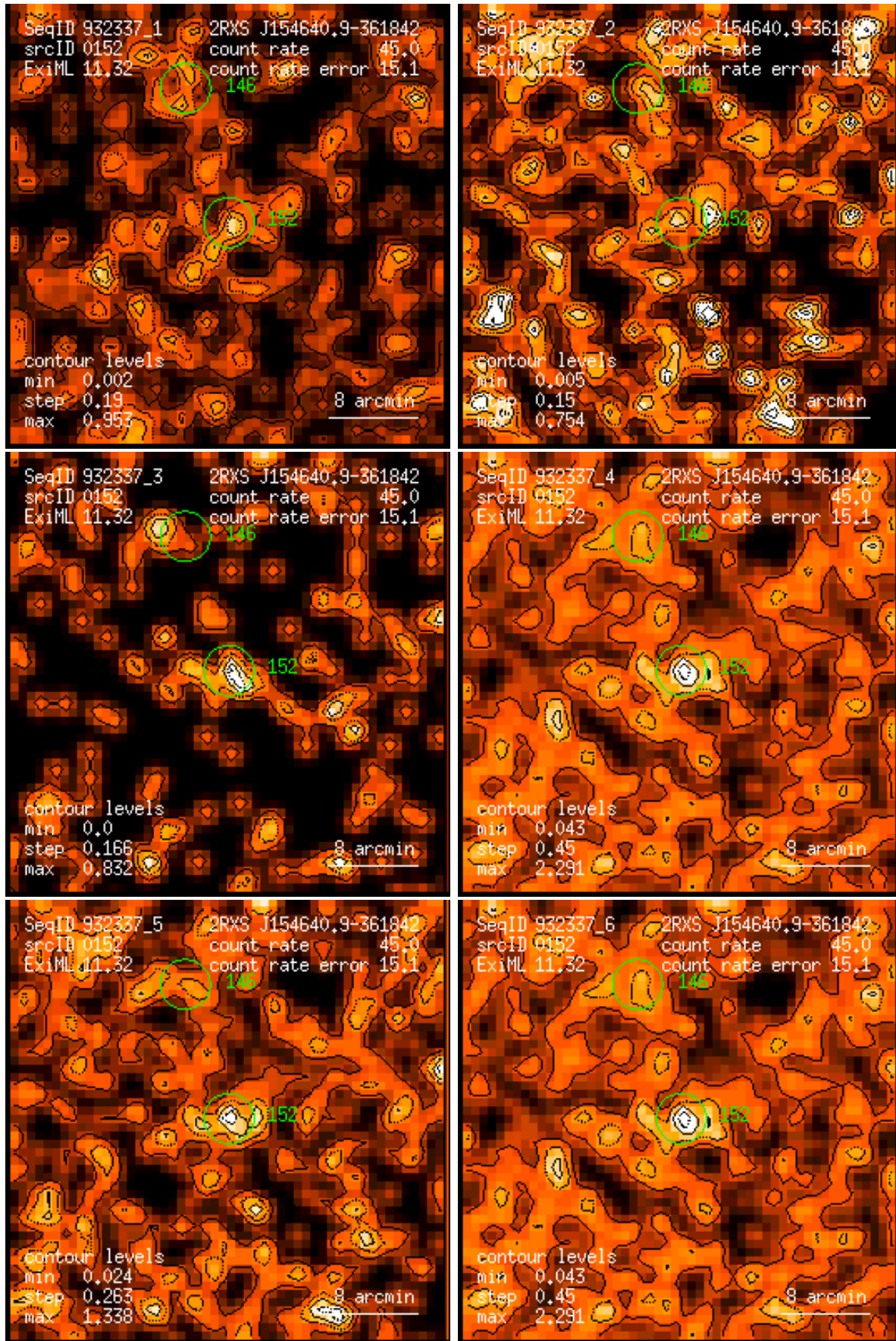
Figure 152: RASS 932337: detection 0152: band rate images, Gaussian filter: (1) PSPC channels 11 – 41, (2) 52 – 90, (3) 91 – 201, (4) 11 – 235, (5) 52 – 201, (6) 11 – 201. Broad band rates in counts/ks. Band rate contour levels in counts/ks/arcmin 2 .
