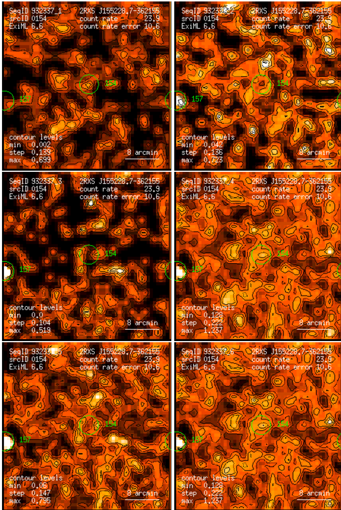
Figure 154: RASS 932337: detection 0154: band rate images, Gaussian filter: (1) PSPC channels 11 – 41, (2) 52 – 90, (3) 91 – 201, (4) 11 – 235, (5) 52 – 201, (6) 11 – 201. Broad band rates in counts/ks. Band rate contour levels in counts/ks/arcmin 2 .
