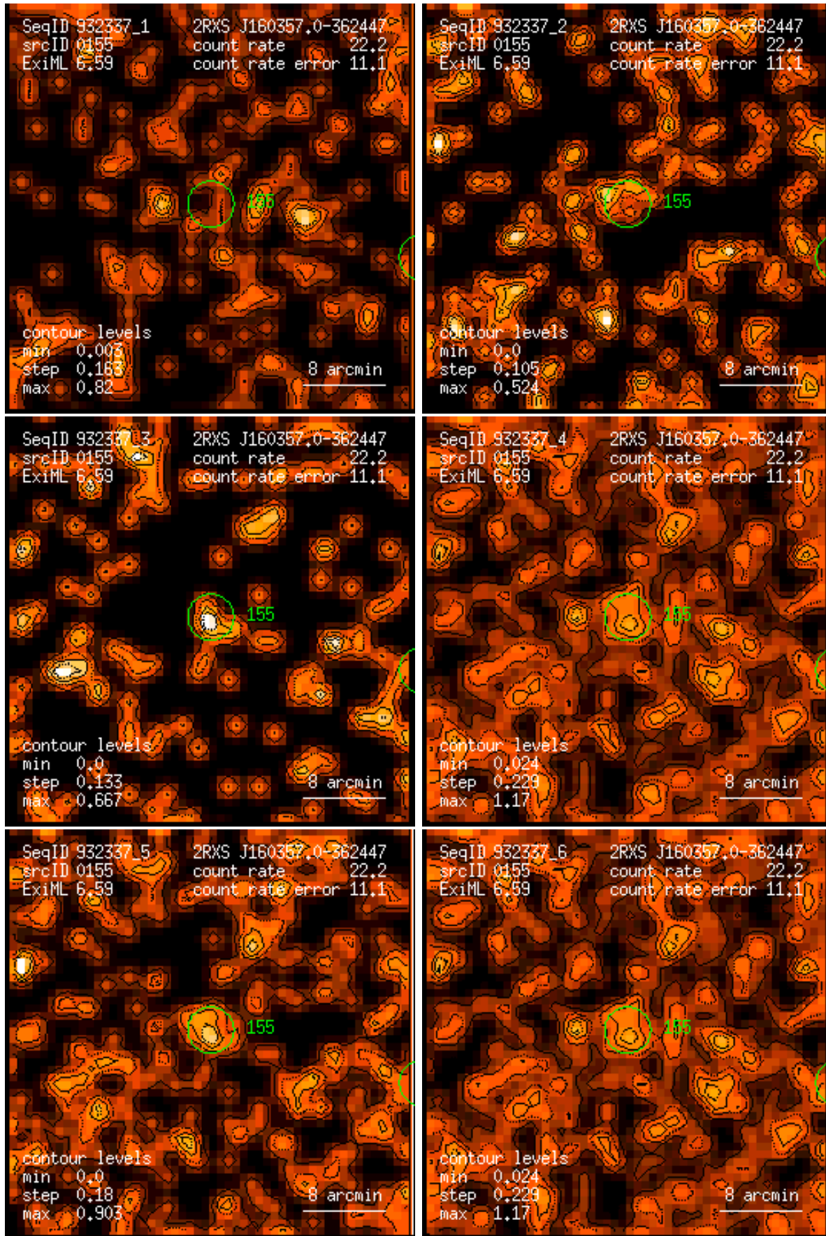
Figure 155: RASS 932337: detection 0155: band rate images, Gaussian filter: (1) PSPC channels 11 – 41, (2) 52 – 90, (3) 91 – 201, (4) 11 – 235, (5) 52 – 201, (6) 11 – 201. Broad band rates in counts/ks. Band rate contour levels in counts/ks/arcmin 2 .
