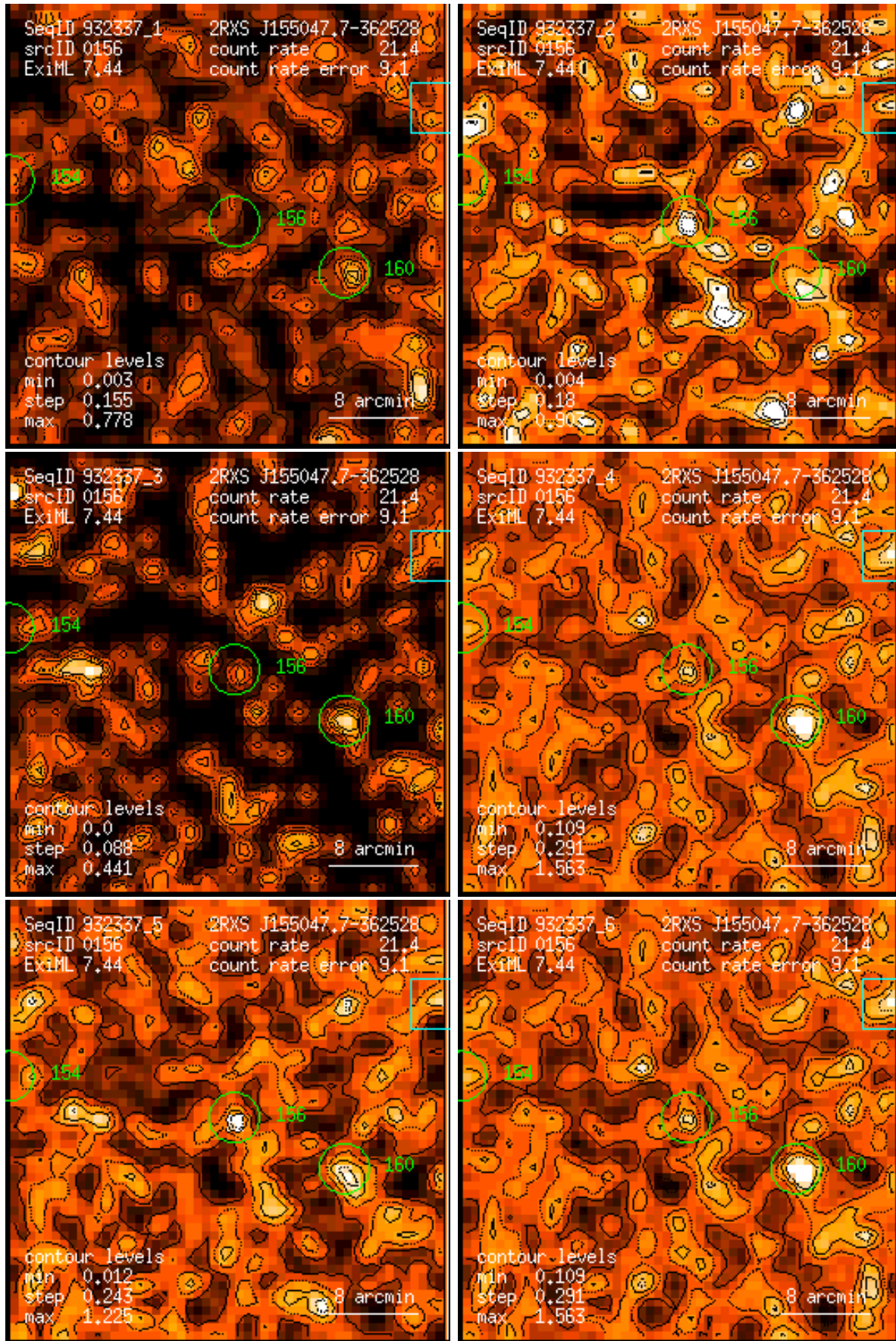
Figure 156: RASS 932337: detection 0156: band rate images, Gaussian filter: (1) PSPC channels 11 – 41, (2) 52 – 90, (3) 91 – 201, (4) 11 – 235, (5) 52 – 201, (6) 11 – 201. Broad band rates in counts/ks. Band rate contour levels in counts/ks/arcmin 2 .
