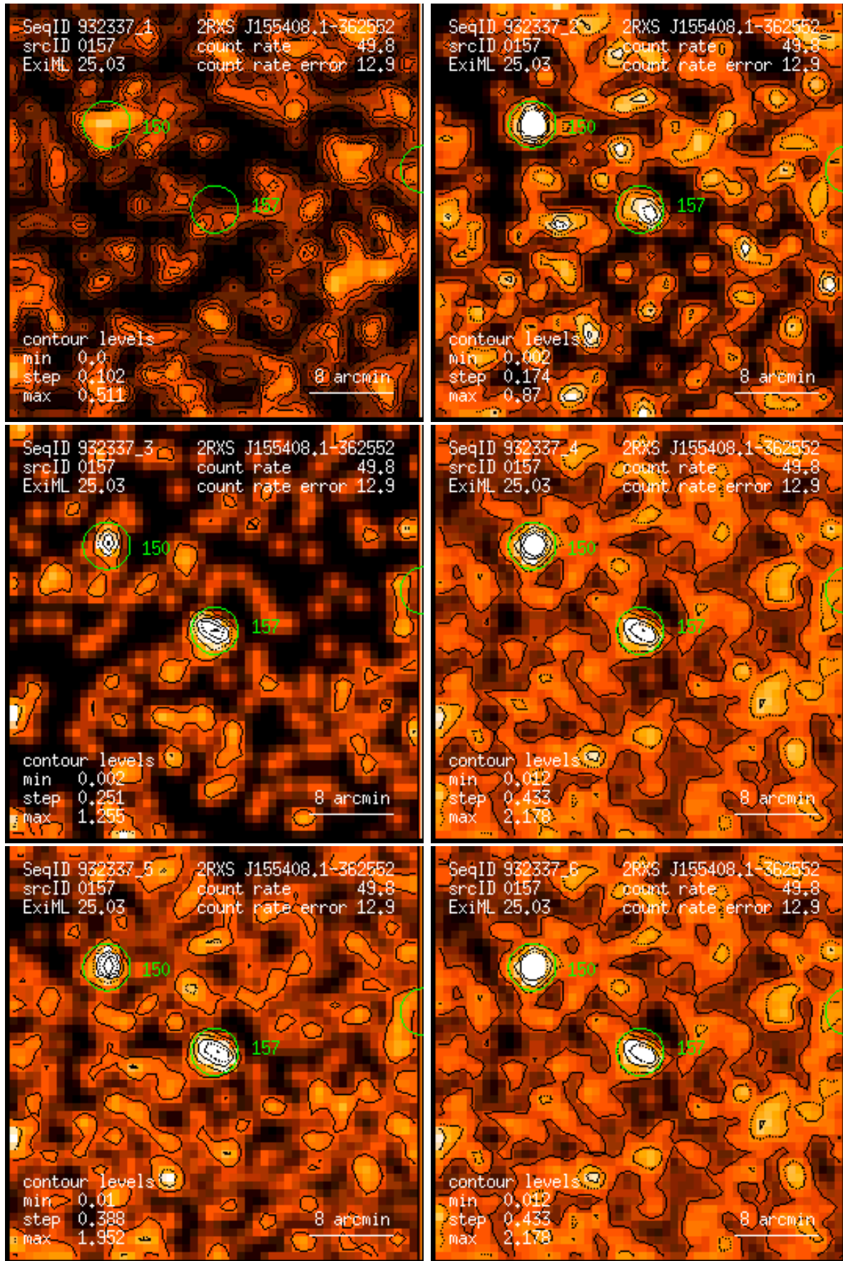
Figure 157: RASS 932337: detection 0157: band rate images, Gaussian filter: (1) PSPC channels 11 – 41, (2) 52 – 90, (3) 91 – 201, (4) 11 – 235, (5) 52 – 201, (6) 11 – 201. Broad band rates in counts/ks. Band rate contour levels in counts/ks/arcmin 2 .
