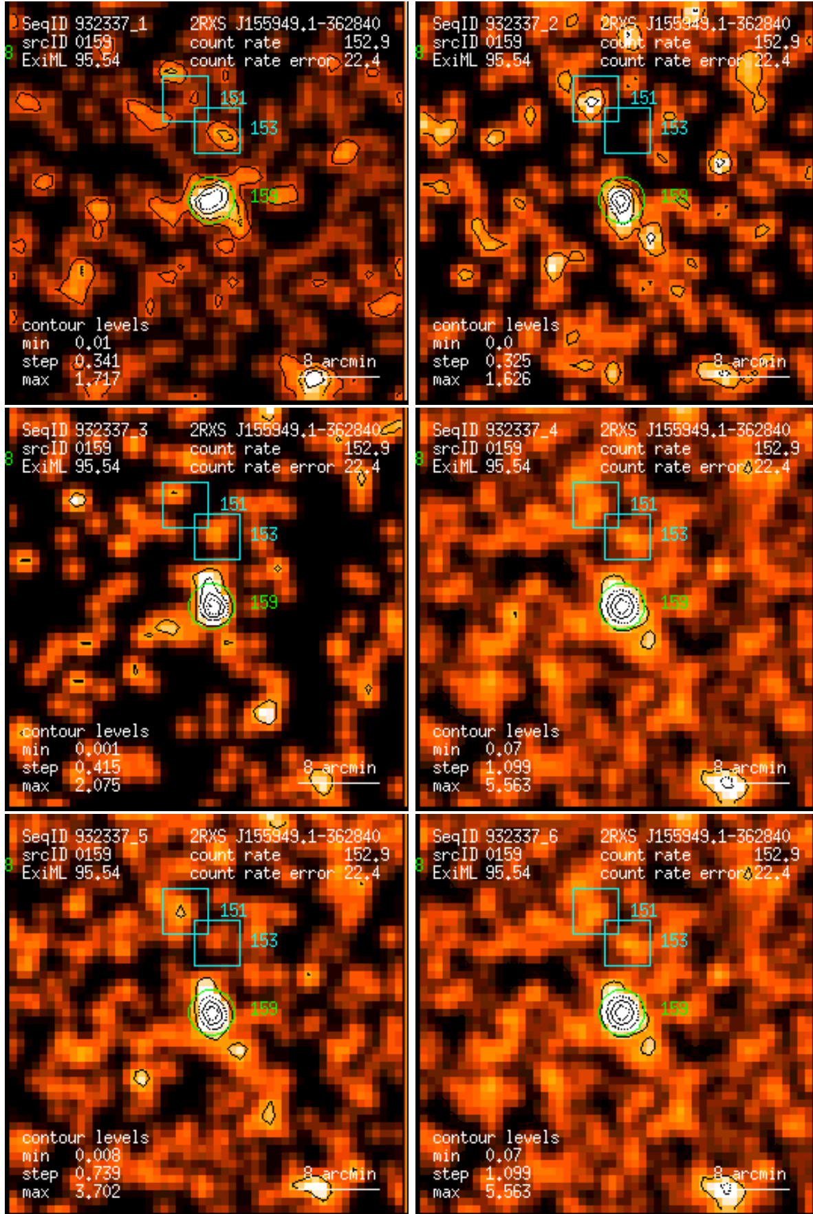
Figure 159: RASS 932337: detection 0159: band rate images, Gaussian filter: (1) PSPC channels 11 – 41, (2) 52 – 90, (3) 91 – 201, (4) 11 – 235, (5) 52 – 201, (6) 11 – 201. Broad band rates in counts/ks. Band rate contour levels in counts/ks/arcmin 2 .
