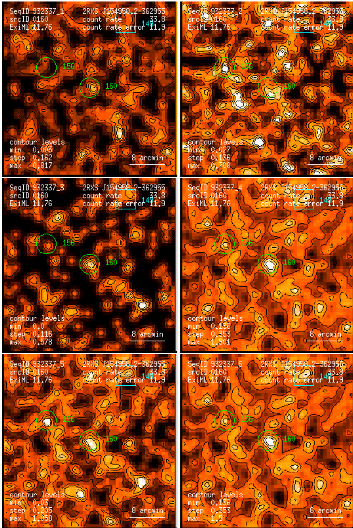
Figure 160: RASS 932337: detection 0160: band rate images, Gaussian filter: (1) PSPC channels 11 – 41, (2) 52 – 90, (3) 91 – 201, (4) 11 – 235, (5) 52 – 201, (6) 11 – 201. Broad band rates in counts/ks. Band rate contour levels in counts/ks/arcmin 2 .
