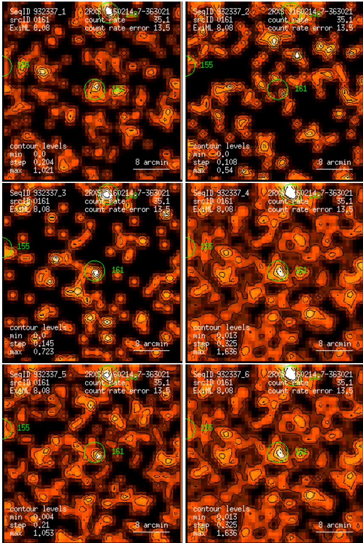
Figure 161: RASS 932337: detection 0161: band rate images, Gaussian filter: (1) PSPC channels 11 – 41, (2) 52 – 90, (3) 91 – 201, (4) 11 – 235, (5) 52 – 201, (6) 11 – 201. Broad band rates in counts/ks. Band rate contour levels in counts/ks/arcmin 2 .
