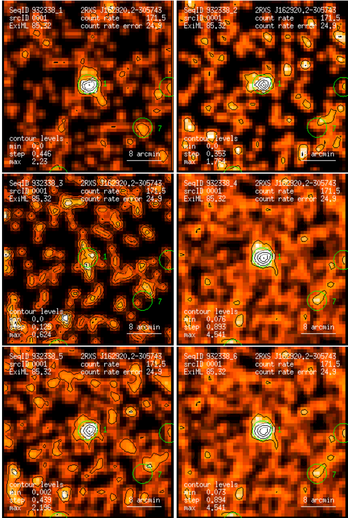
Figure 1: RASS 932338: detection 0001: band rate images, Gaussian filter: (1) PSPC channels 11 – 41, (2) 52 – 90, (3) 91 – 201, (4) 11 – 235, (5) 52 – 201, (6) 11 – 201. Broad band rates in counts/ks. Band rate contour levels in counts/ks/arcmin 2 .
