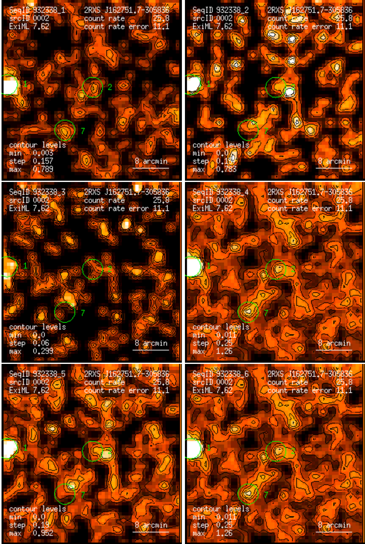
Figure 2: RASS 932338: detection 0002: band rate images, Gaussian filter: (1) PSPC channels 11 – 41, (2) 52 – 90, (3) 91 – 201, (4) 11 – 235, (5) 52 – 201, (6) 11 – 201. Broad band rates in counts/ks. Band rate contour levels in counts/ks/arcmin 2 .
