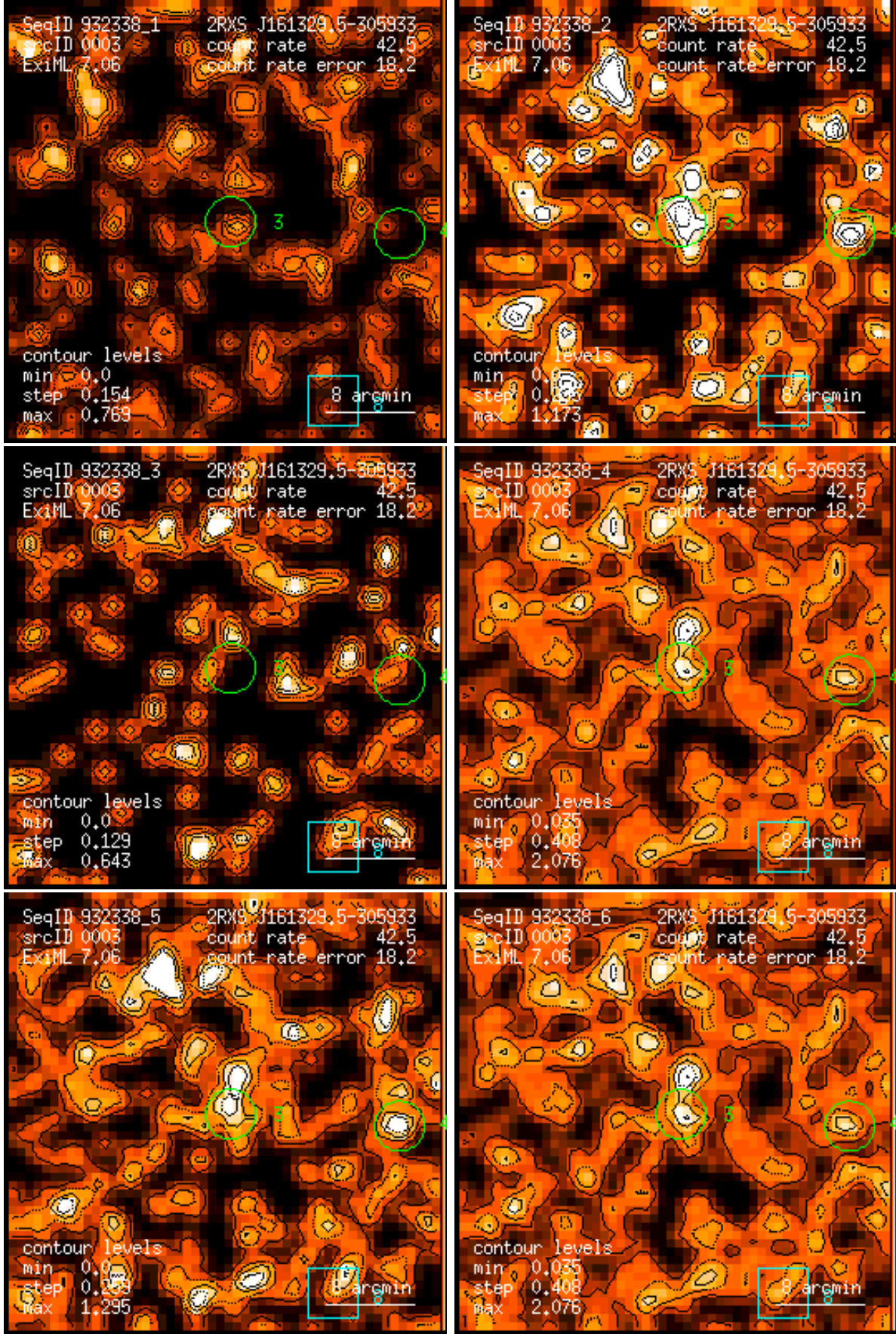
Figure 3: RASS 932338: detection 0003: band rate images, Gaussian filter: (1) PSPC channels 11 – 41, (2) 52 – 90, (3) 91 – 201, (4) 11 – 235, (5) 52 – 201, (6) 11 – 201. Broad band rates in counts/ks. Band rate contour levels in counts/ks/arcmin 2 .
