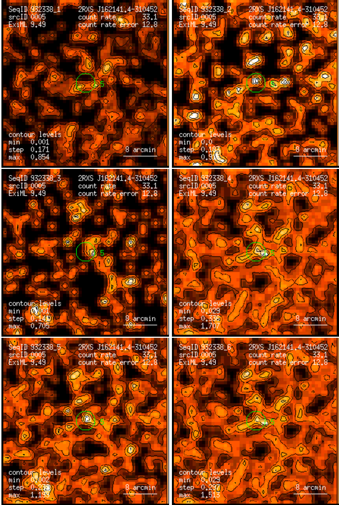
Figure 5: RASS 932338: detection 0005: band rate images, Gaussian filter: (1) PSPC channels 11 – 41, (2) 52 – 90, (3) 91 – 201, (4) 11 – 235, (5) 52 – 201, (6) 11 – 201. Broad band rates in counts/ks. Band rate contour levels in counts/ks/arcmin 2 .
