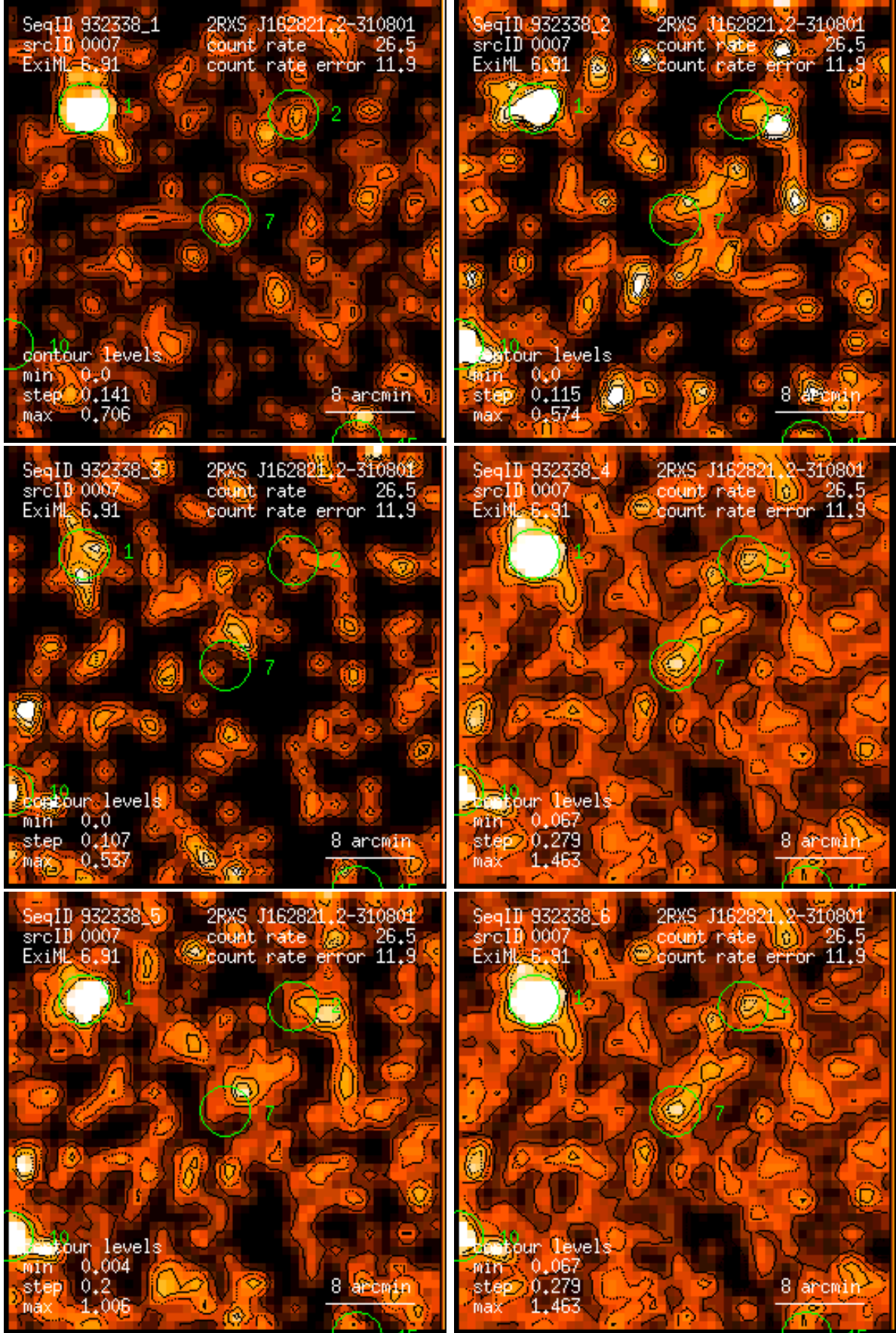
Figure 7: RASS 932338: detection 0007: band rate images, Gaussian filter: (1) PSPC channels 11 – 41, (2) 52 – 90, (3) 91 – 201, (4) 11 – 235, (5) 52 – 201, (6) 11 – 201. Broad band rates in counts/ks. Band rate contour levels in counts/ks/arcmin 2 .
