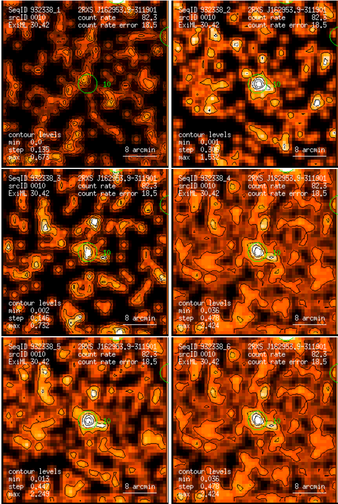
Figure 10: RASS 932338: detection 0010: band rate images, Gaussian filter: (1) PSPC channels 11 – 41, (2) 52 – 90, (3) 91 – 201, (4) 11 – 235, (5) 52 – 201, (6) 11 – 201. Broad band rates in counts/ks. Band rate contour levels in counts/ks/arcmin 2 .
