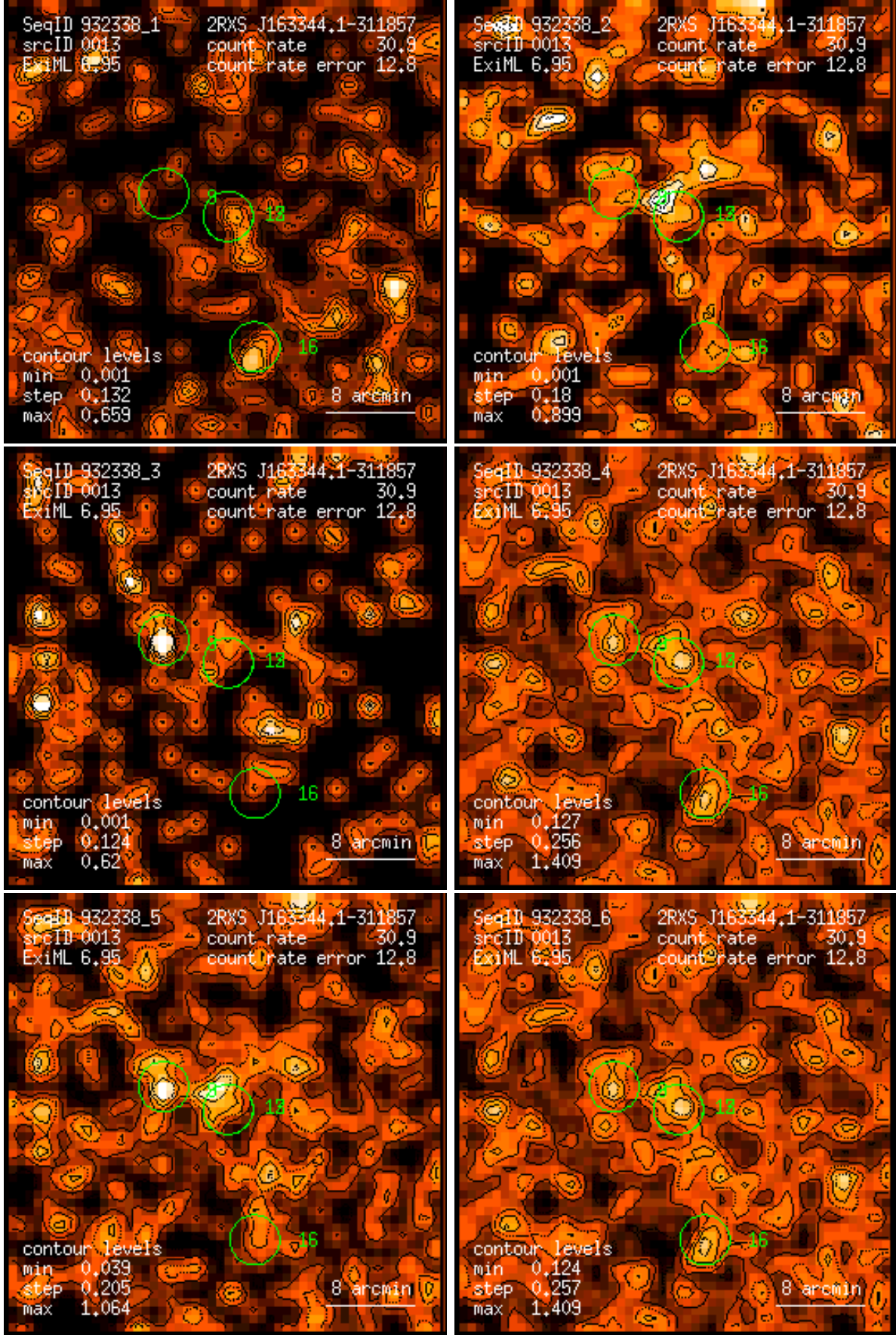
Figure 13: RASS 932338: detection 0013: band rate images, Gaussian filter: (1) PSPC channels 11 – 41, (2) 52 – 90, (3) 91 – 201, (4) 11 – 235, (5) 52 – 201, (6) 11 – 201. Broad band rates in counts/ks. Band rate contour levels in counts/ks/arcmin 2 .
