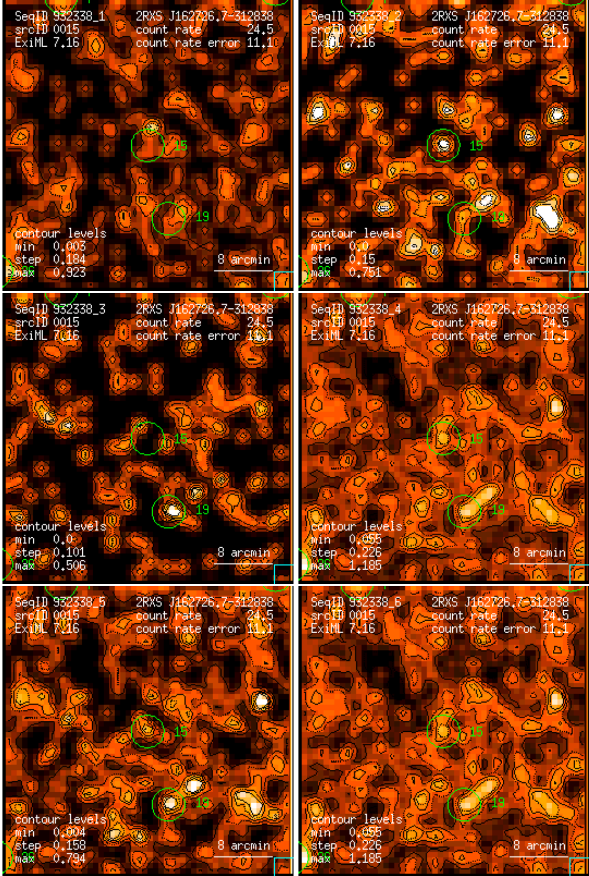
Figure 15: RASS 932338: detection 0015: band rate images, Gaussian filter: (1) PSPC channels 11 – 41, (2) 52 – 90, (3) 91 – 201, (4) 11 – 235, (5) 52 – 201, (6) 11 – 201. Broad band rates in counts/ks. Band rate contour levels in counts/ks/arcmin 2 .
