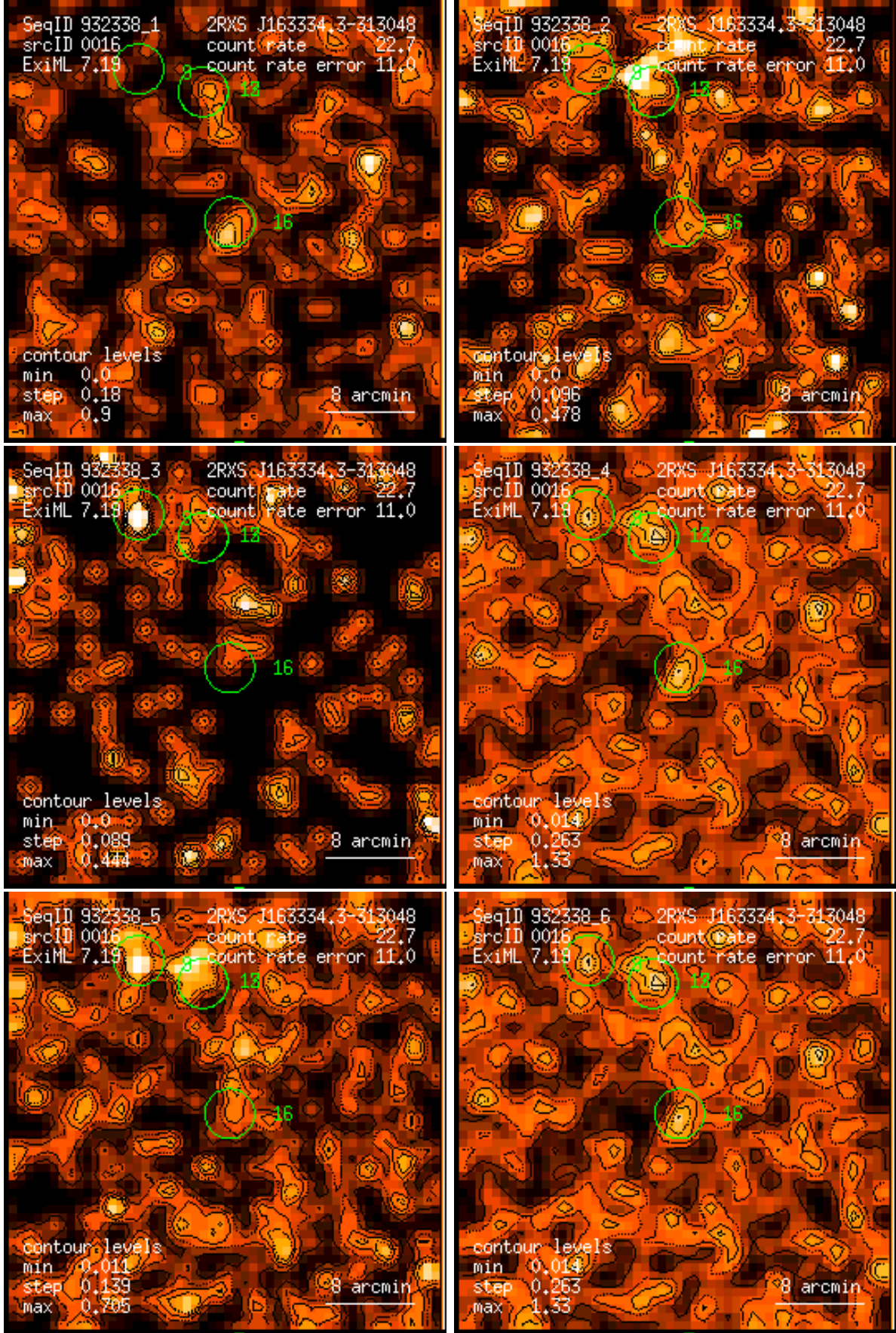
Figure 16: RASS 932338: detection 0016: band rate images, Gaussian filter: (1) PSPC channels 11 – 41, (2) 52 – 90, (3) 91 – 201, (4) 11 – 235, (5) 52 – 201, (6) 11 – 201. Broad band rates in counts/ks. Band rate contour levels in counts/ks/arcmin 2 .
