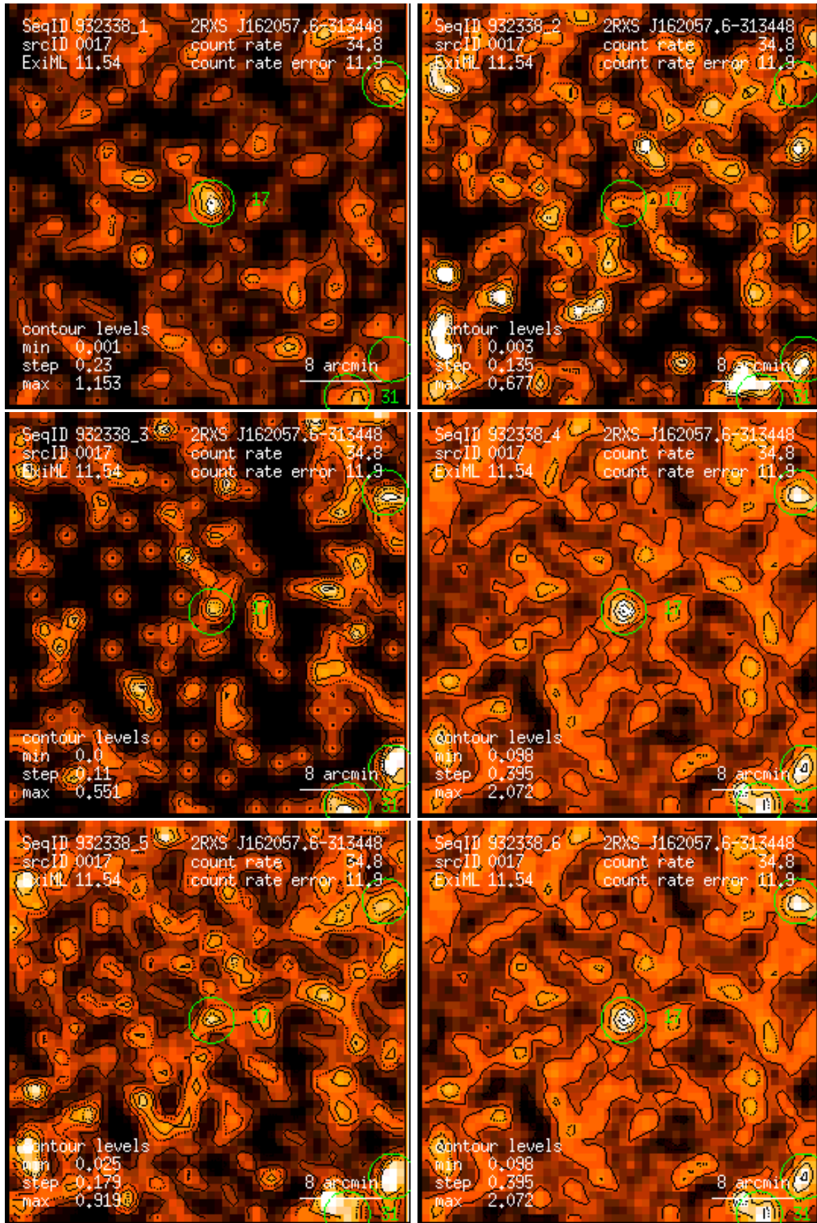
Figure 17: RASS 932338: detection 0017: band rate images, Gaussian filter: (1) PSPC channels 11 – 41, (2) 52 – 90, (3) 91 – 201, (4) 11 – 235, (5) 52 – 201, (6) 11 – 201. Broad band rates in counts/ks. Band rate contour levels in counts/ks/arcmin 2 .
