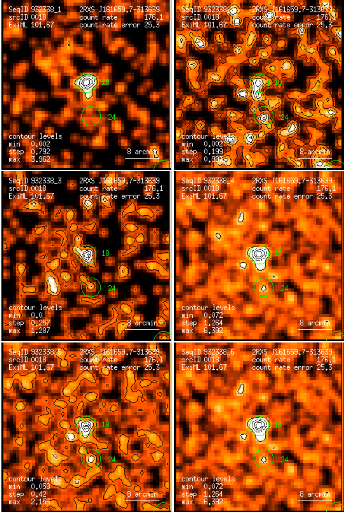
Figure 18: RASS 932338: detection 0018: band rate images, Gaussian filter: (1) PSPC channels 11 – 41, (2) 52 – 90, (3) 91 – 201, (4) 11 – 235, (5) 52 – 201, (6) 11 – 201. Broad band rates in counts/ks. Band rate contour levels in counts/ks/arcmin 2 .
