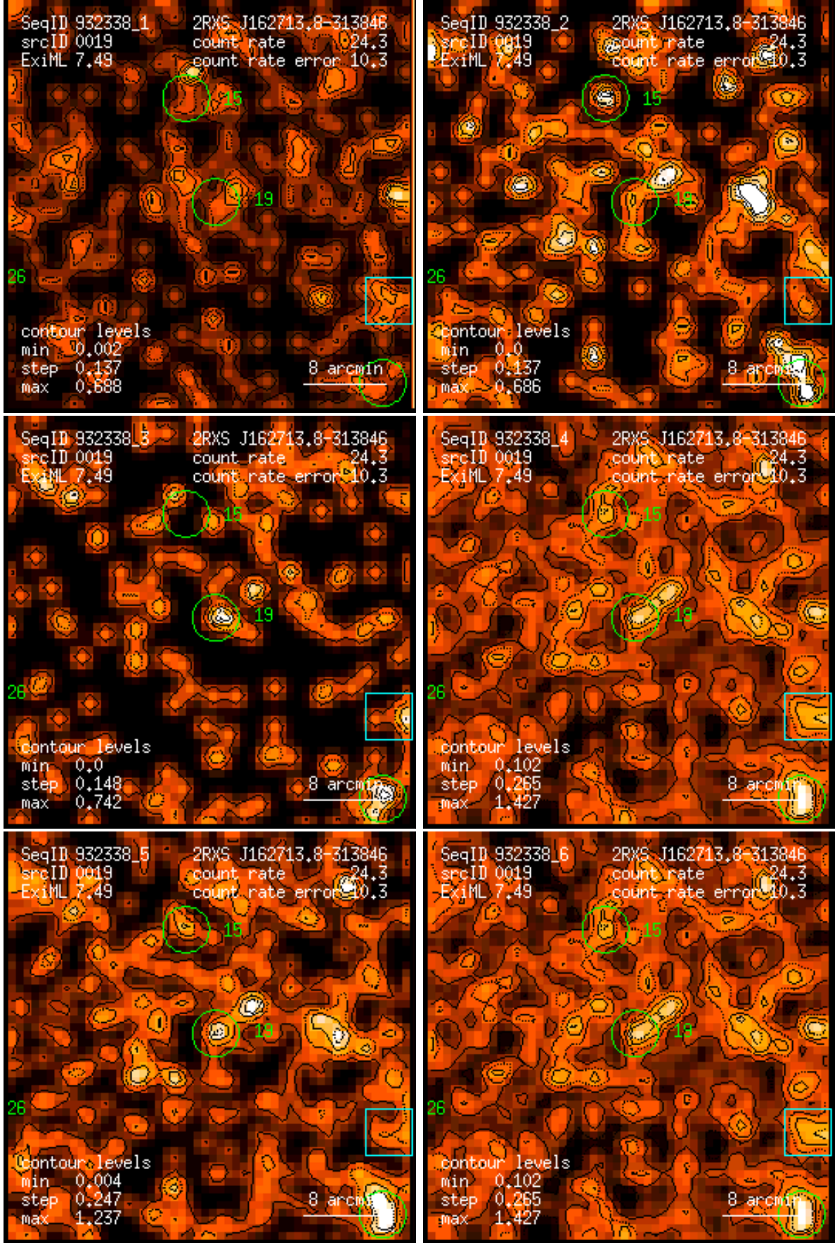
Figure 19: RASS 932338: detection 0019: band rate images, Gaussian filter: (1) PSPC channels 11 – 41, (2) 52 – 90, (3) 91 – 201, (4) 11 – 235, (5) 52 – 201, (6) 11 – 201. Broad band rates in counts/ks. Band rate contour levels in counts/ks/arcmin 2 .
