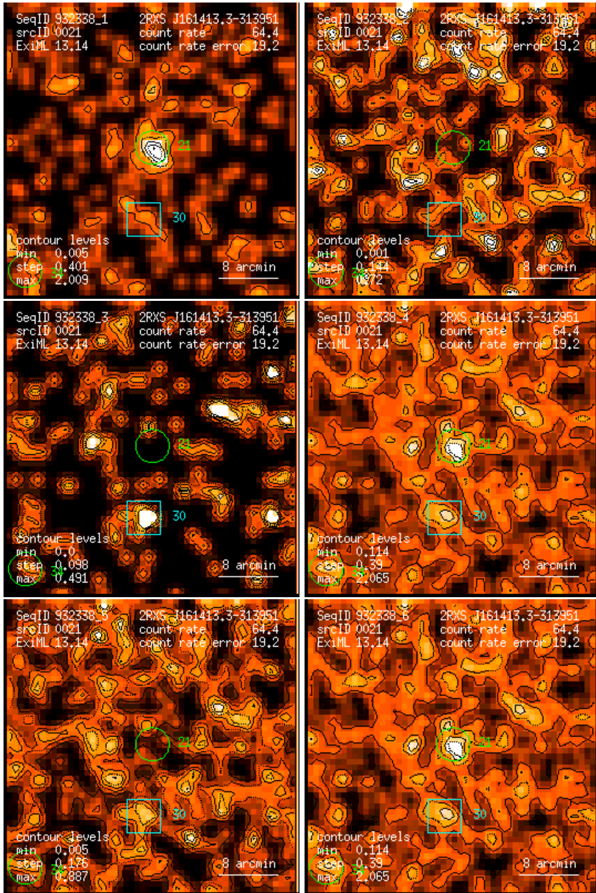
Figure 21: RASS 932338: detection 0021: band rate images, Gaussian filter: (1) PSPC channels 11 – 41, (2) 52 – 90, (3) 91 – 201, (4) 11 – 235, (5) 52 – 201, (6) 11 – 201. Broad band rates in counts/ks. Band rate contour levels in counts/ks/arcmin 2 .
