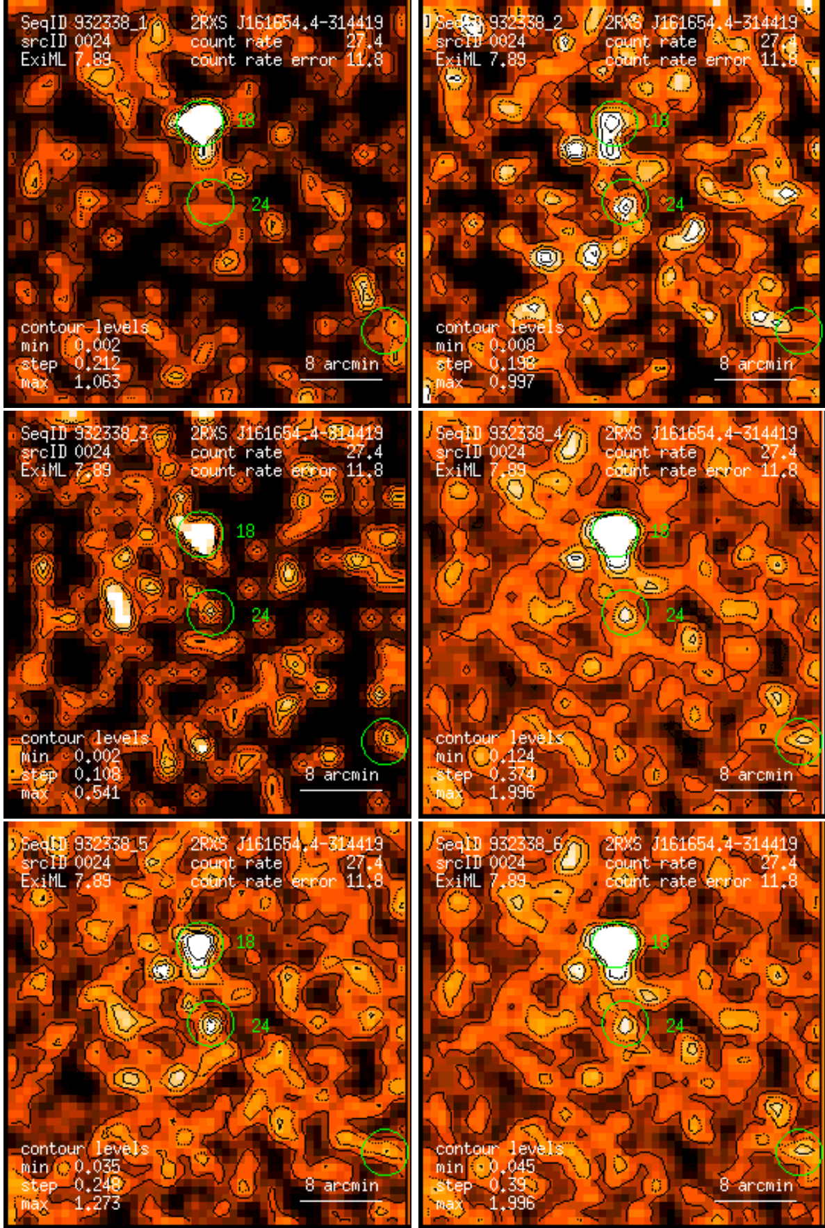
Figure 24: RASS 932338: detection 0024: band rate images, Gaussian filter: (1) PSPC channels 11 – 41, (2) 52 – 90, (3) 91 – 201, (4) 11 – 235, (5) 52 – 201, (6) 11 – 201. Broad band rates in counts/ks. Band rate contour levels in counts/ks/arcmin 2 .
