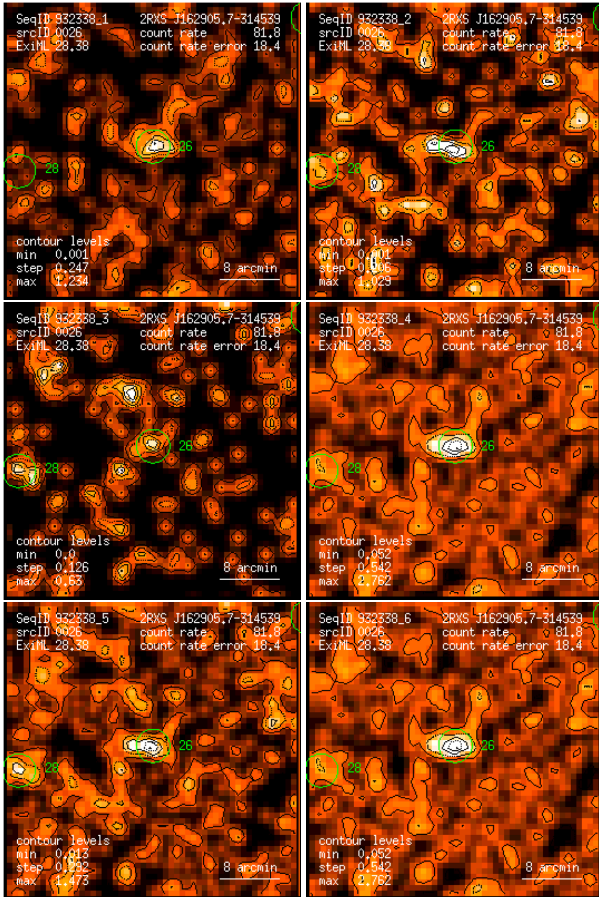
Figure 26: RASS 932338: detection 0026: band rate images, Gaussian filter: (1) PSPC channels 11 – 41, (2) 52 – 90, (3) 91 – 201, (4) 11 – 235, (5) 52 – 201, (6) 11 – 201. Broad band rates in counts/ks. Band rate contour levels in counts/ks/arcmin 2 .
