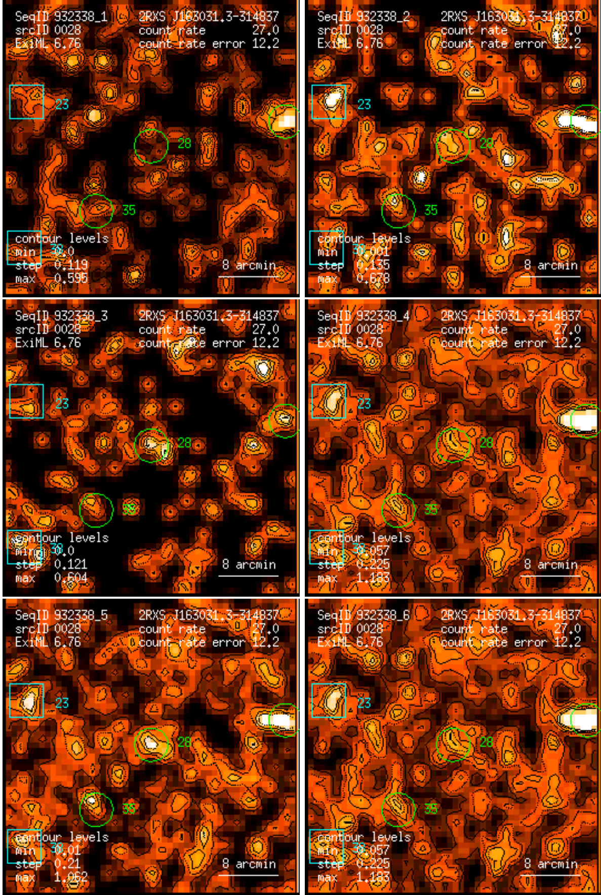
Figure 28: RASS 932338: detection 0028: band rate images, Gaussian filter: (1) PSPC channels 11 – 41, (2) 52 – 90, (3) 91 – 201, (4) 11 – 235, (5) 52 – 201, (6) 11 – 201. Broad band rates in counts/ks. Band rate contour levels in counts/ks/arcmin 2 .
