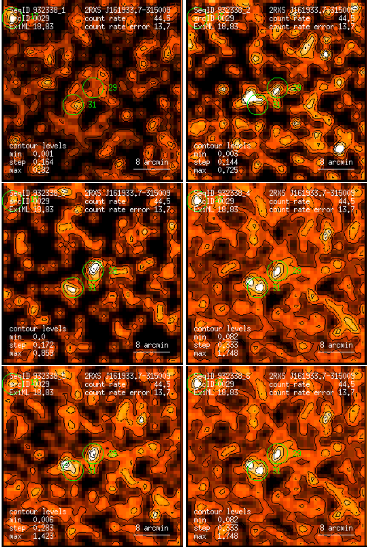
Figure 29: RASS 932338: detection 0029: band rate images, Gaussian filter: (1) PSPC channels 11 – 41, (2) 52 – 90, (3) 91 – 201, (4) 11 – 235, (5) 52 – 201, (6) 11 – 201. Broad band rates in counts/ks. Band rate contour levels in counts/ks/arcmin 2 .
