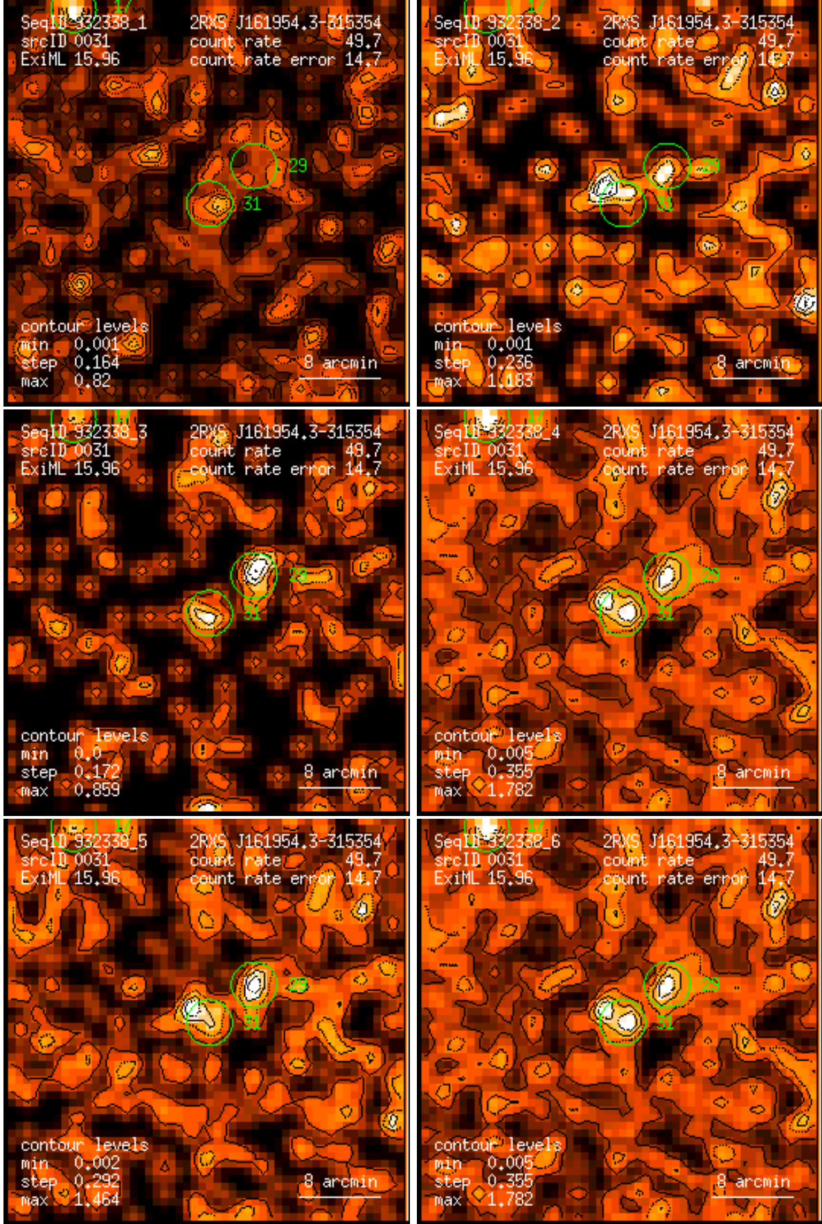
Figure 31: RASS 932338: detection 0031: band rate images, Gaussian filter: (1) PSPC channels 11 – 41, (2) 52 – 90, (3) 91 – 201, (4) 11 – 235, (5) 52 – 201, (6) 11 – 201. Broad band rates in counts/ks. Band rate contour levels in counts/ks/arcmin 2 .
