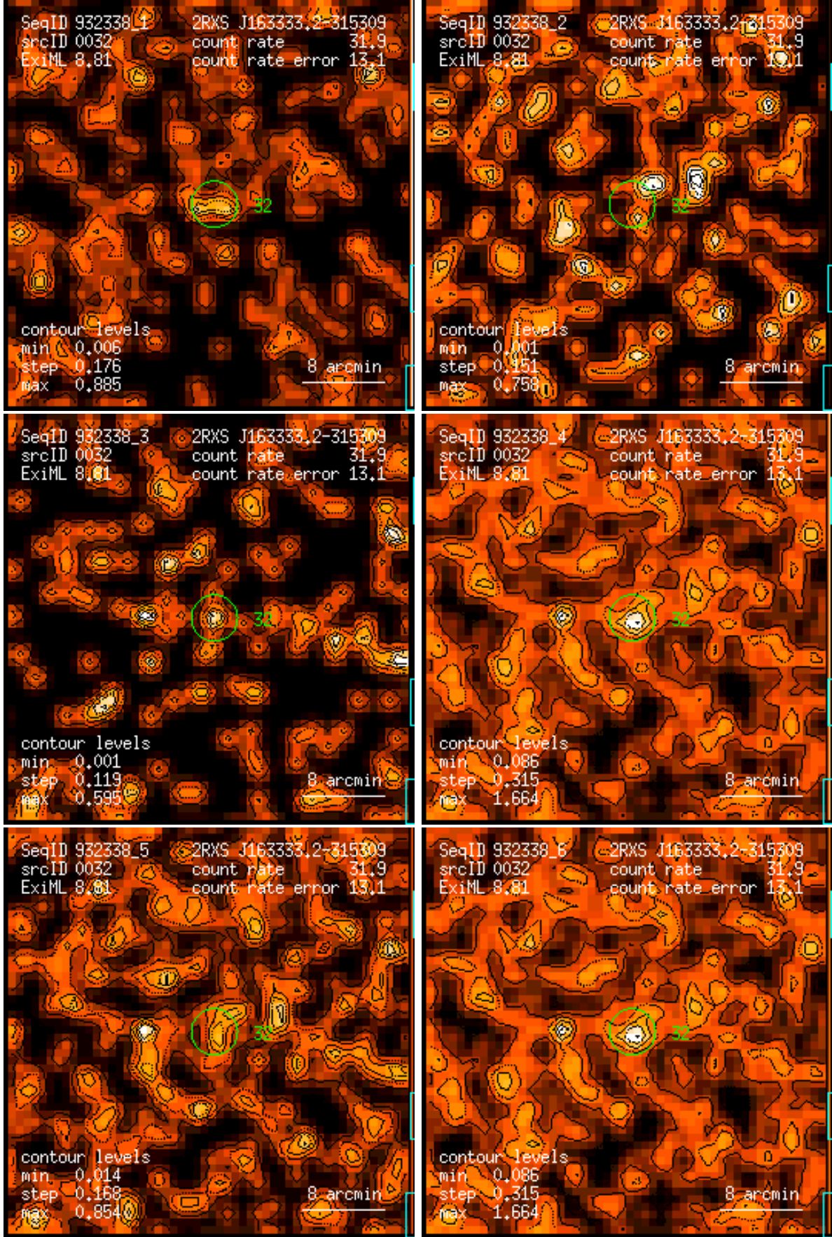
Figure 32: RASS 932338: detection 0032: band rate images, Gaussian filter: (1) PSPC channels 11 – 41, (2) 52 – 90, (3) 91 – 201, (4) 11 – 235, (5) 52 – 201, (6) 11 – 201. Broad band rates in counts/ks. Band rate contour levels in counts/ks/arcmin 2 .
