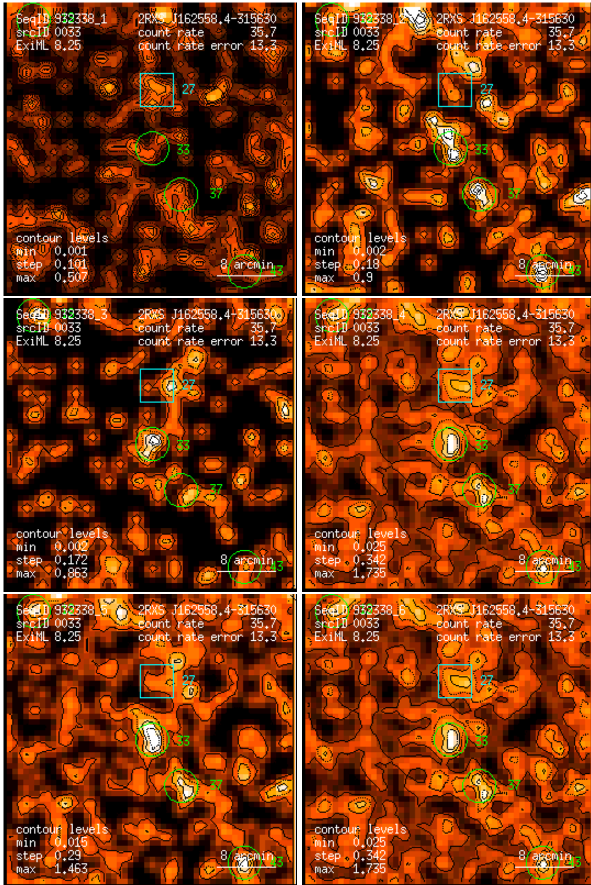
Figure 33: RASS 932338: detection 0033: band rate images, Gaussian filter: (1) PSPC channels 11 – 41, (2) 52 – 90, (3) 91 – 201, (4) 11 – 235, (5) 52 – 201, (6) 11 – 201. Broad band rates in counts/ks. Band rate contour levels in counts/ks/arcmin 2 .
