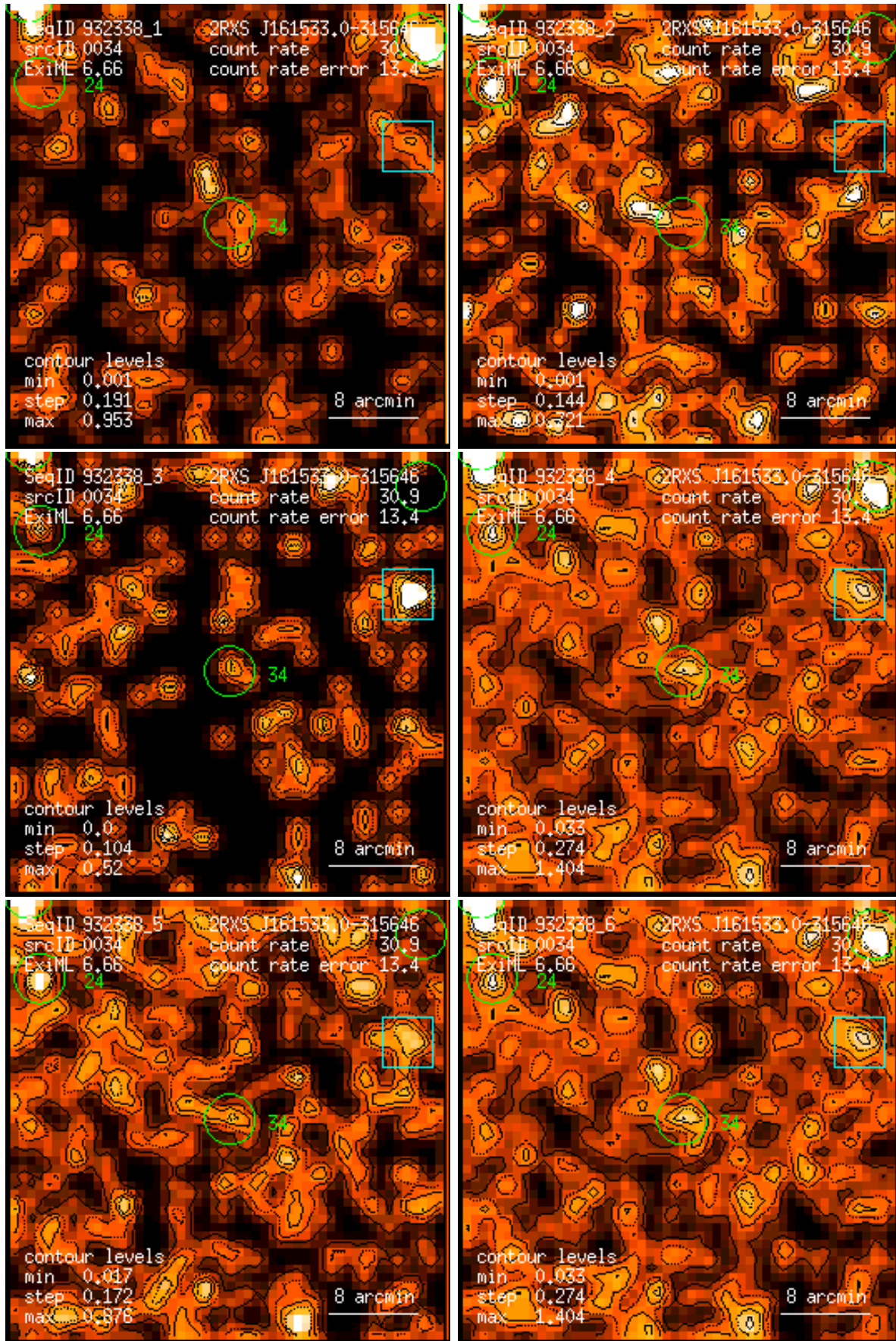
Figure 34: RASS 932338: detection 0034: band rate images, Gaussian filter: (1) PSPC channels 11 – 41, (2) 52 – 90, (3) 91 – 201, (4) 11 – 235, (5) 52 – 201, (6) 11 – 201. Broad band rates in counts/ks. Band rate contour levels in counts/ks/arcmin 2 .
