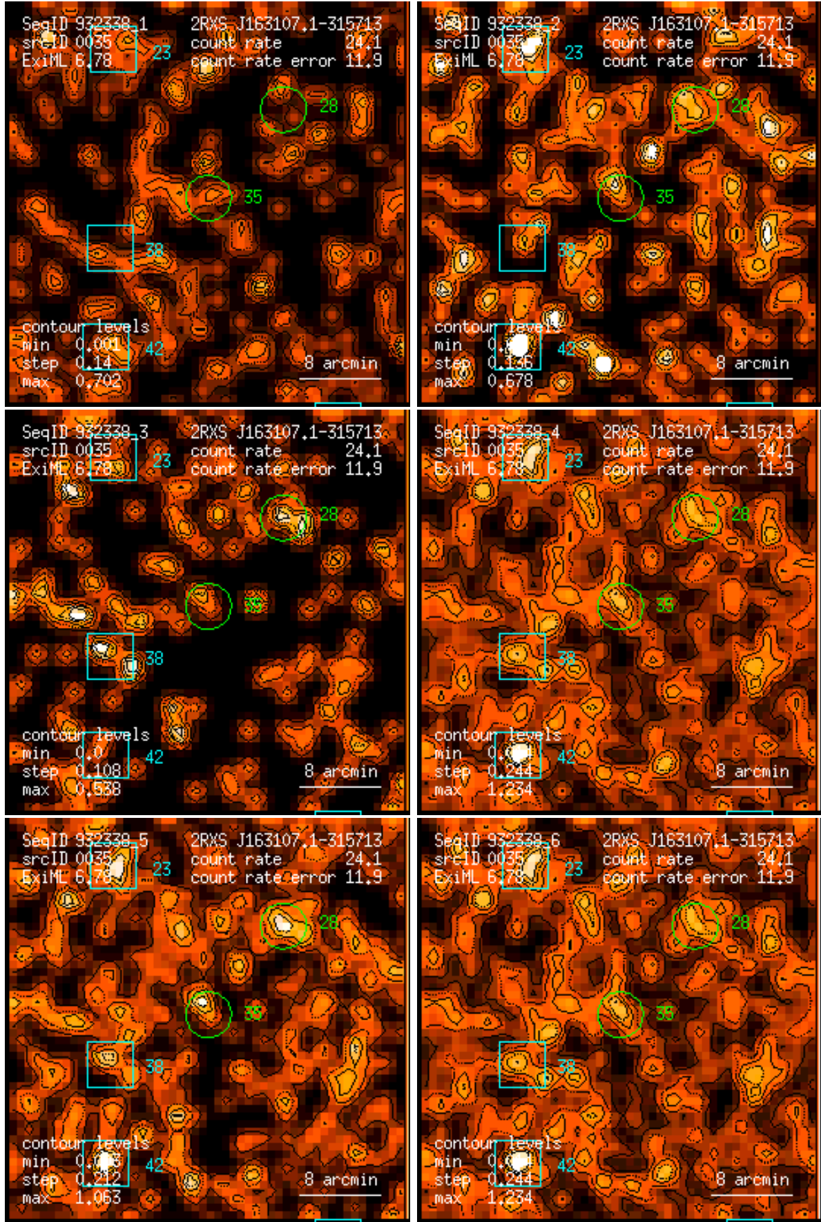
Figure 35: RASS 932338: detection 0035: band rate images, Gaussian filter: (1) PSPC channels 11 – 41, (2) 52 – 90, (3) 91 – 201, (4) 11 – 235, (5) 52 – 201, (6) 11 – 201. Broad band rates in counts/ks. Band rate contour levels in counts/ks/arcmin 2 .
