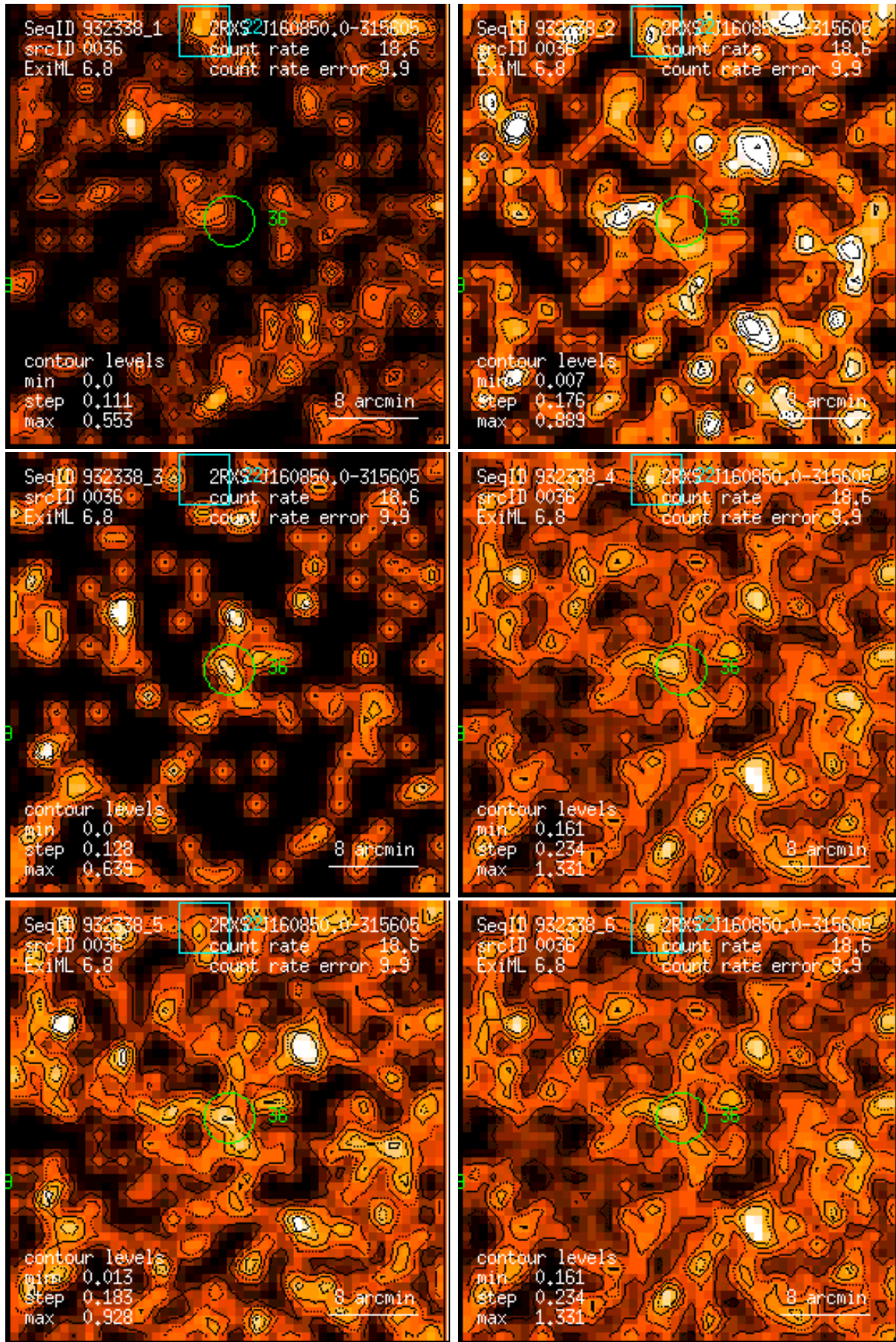
Figure 36: RASS 932338: detection 0036: band rate images, Gaussian filter: (1) PSPC channels 11 – 41, (2) 52 – 90, (3) 91 – 201, (4) 11 – 235, (5) 52 – 201, (6) 11 – 201. Broad band rates in counts/ks. Band rate contour levels in counts/ks/arcmin 2 .
