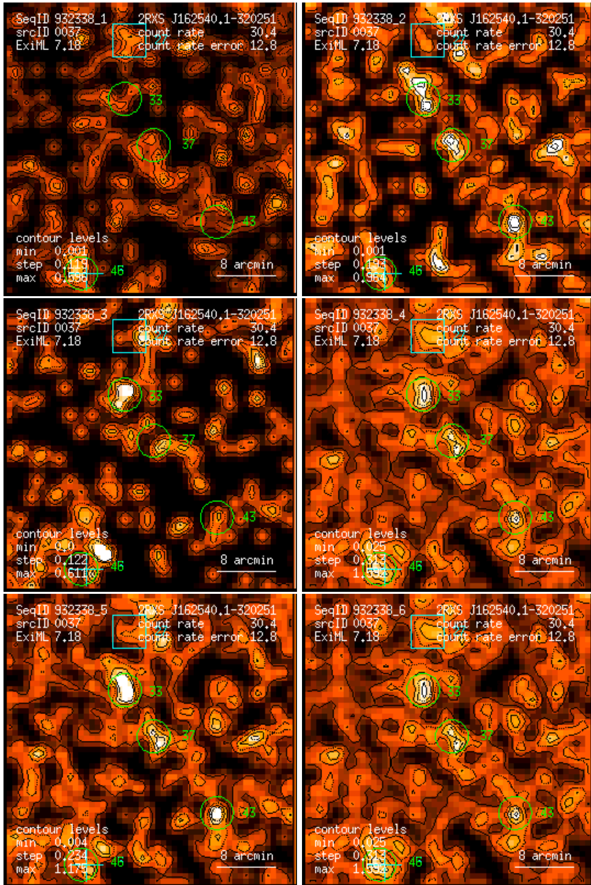
Figure 37: RASS 932338: detection 0037: band rate images, Gaussian filter: (1) PSPC channels 11 – 41, (2) 52 – 90, (3) 91 – 201, (4) 11 – 235, (5) 52 – 201, (6) 11 – 201. Broad band rates in counts/ks. Band rate contour levels in counts/ks/arcmin 2 .
