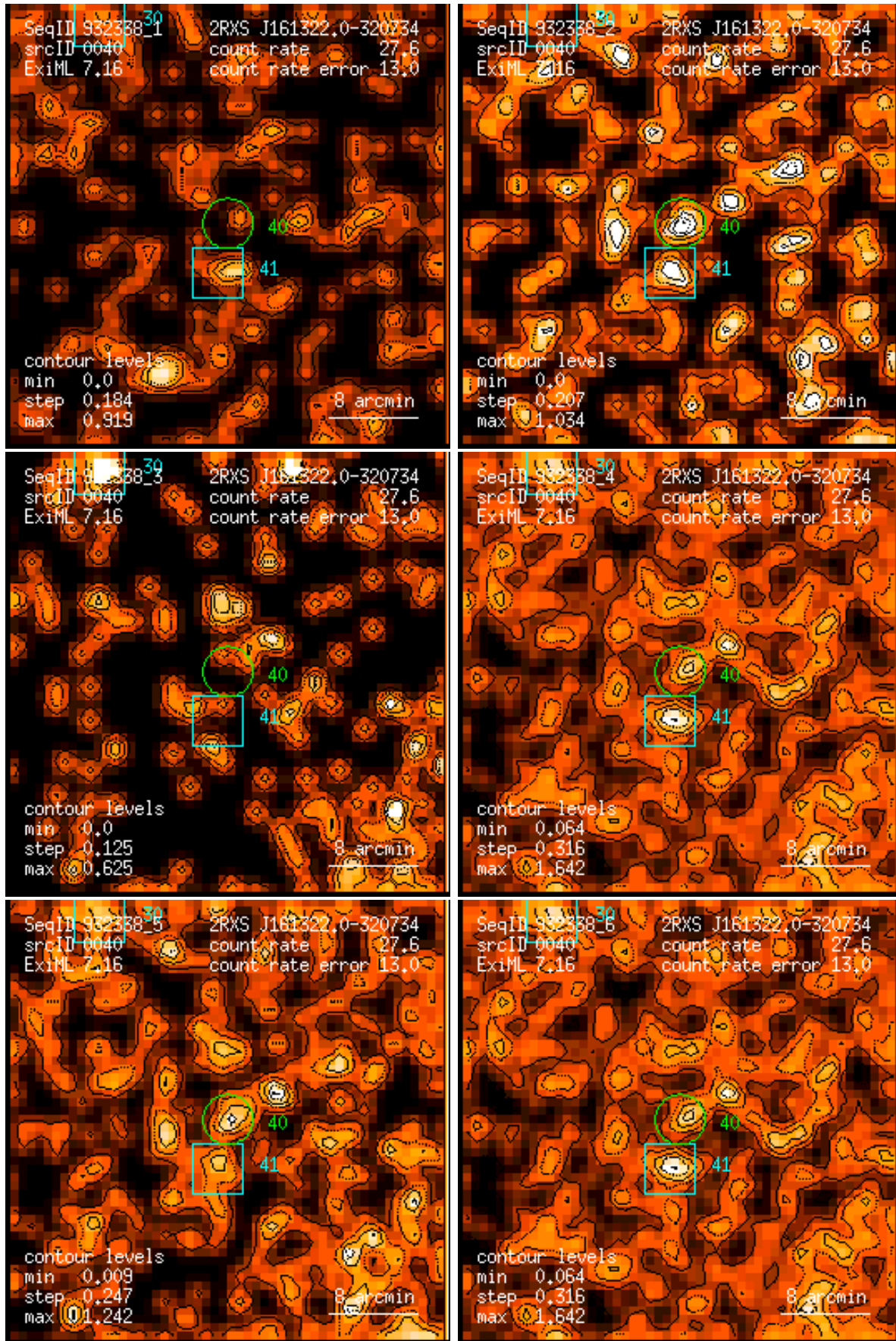
Figure 40: RASS 932338: detection 0040: band rate images, Gaussian filter: (1) PSPC channels 11 – 41, (2) 52 – 90, (3) 91 – 201, (4) 11 – 235, (5) 52 – 201, (6) 11 – 201. Broad band rates in counts/ks. Band rate contour levels in counts/ks/arcmin 2 .
