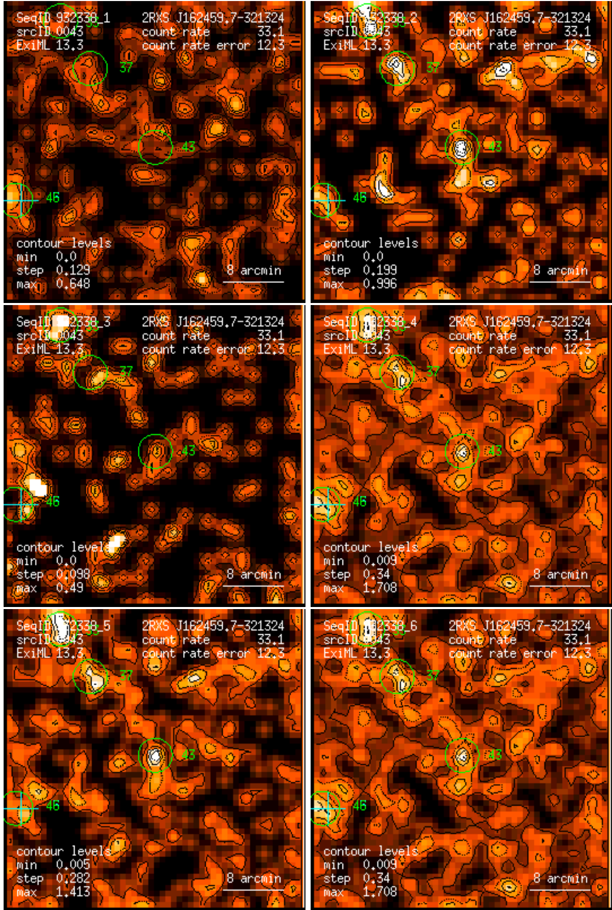
Figure 43: RASS 932338: detection 0043: band rate images, Gaussian filter: (1) PSPC channels 11 – 41, (2) 52 – 90, (3) 91 – 201, (4) 11 – 235, (5) 52 – 201, (6) 11 – 201. Broad band rates in counts/ks. Band rate contour levels in counts/ks/arcmin 2 .
