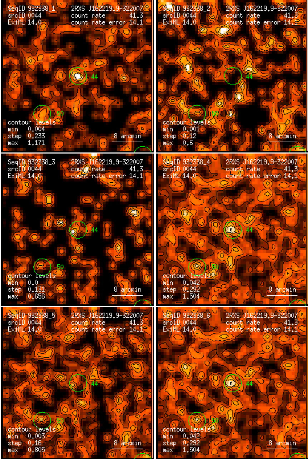
Figure 44: RASS 932338: detection 0044: band rate images, Gaussian filter: (1) PSPC channels 11 – 41, (2) 52 – 90, (3) 91 – 201, (4) 11 – 235, (5) 52 – 201, (6) 11 – 201. Broad band rates in counts/ks. Band rate contour levels in counts/ks/arcmin 2 .
